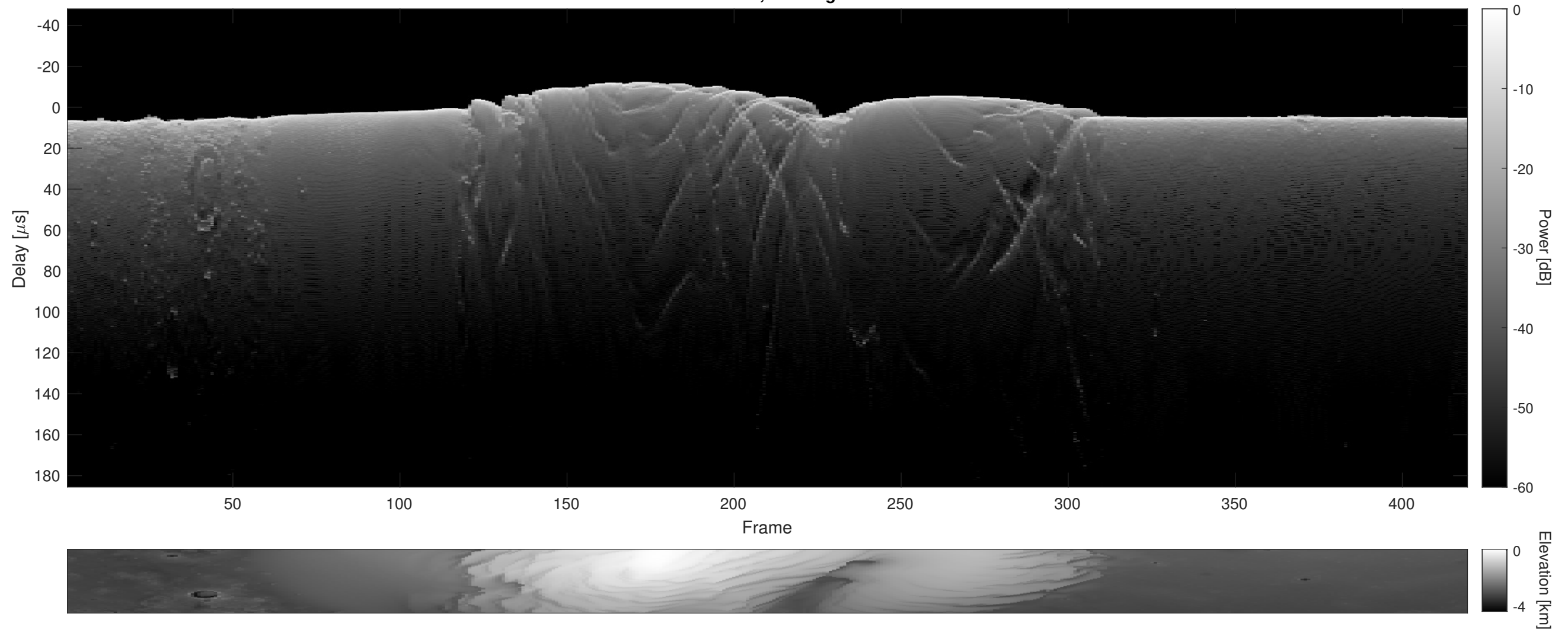
Orbit 17959, Cluttergram
