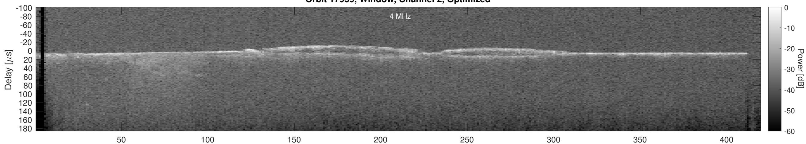
Orbit 17959, Cluttergram
