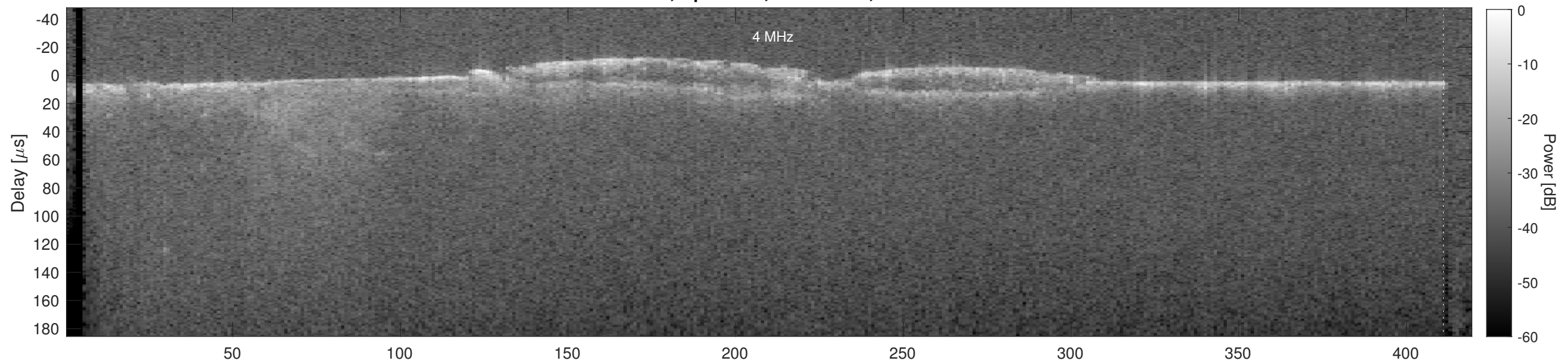
Orbit 17959, Cluttergram
