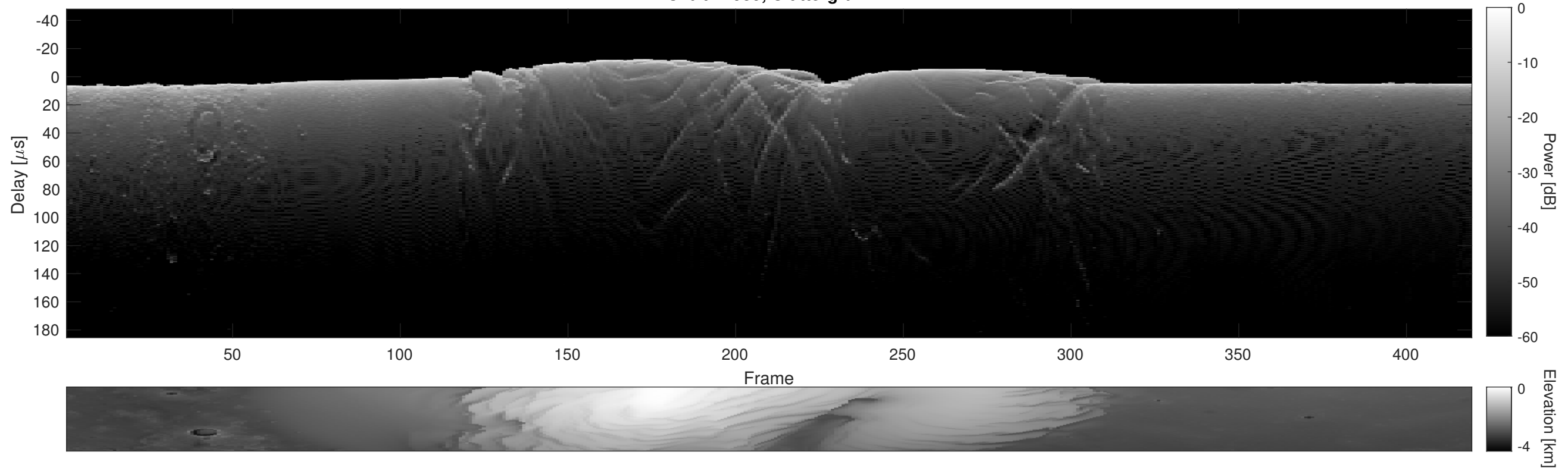
Orbit 17959, Cluttergram
