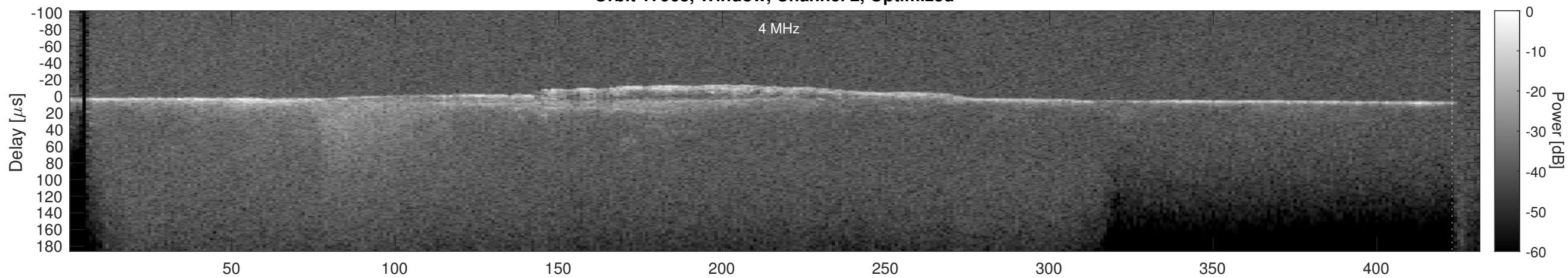
Orbit 17963, Cluttergram
