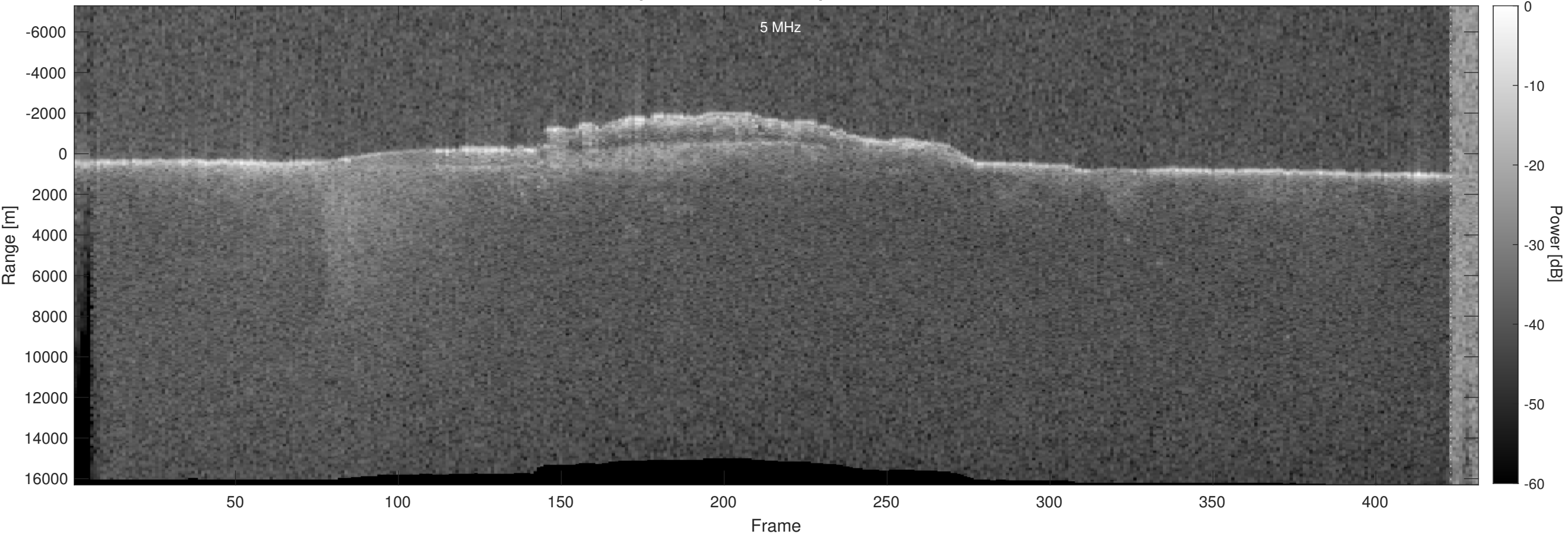
Orbit 17963, Optimized, Window, Depth-Corrected, Channel 2
