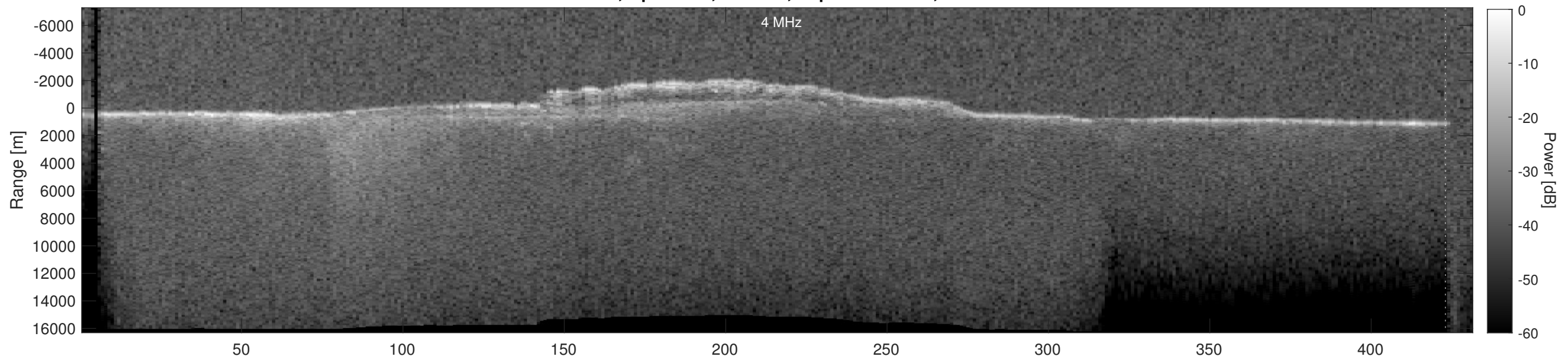
Orbit 17963, Depth-Corrected Cluttergram
