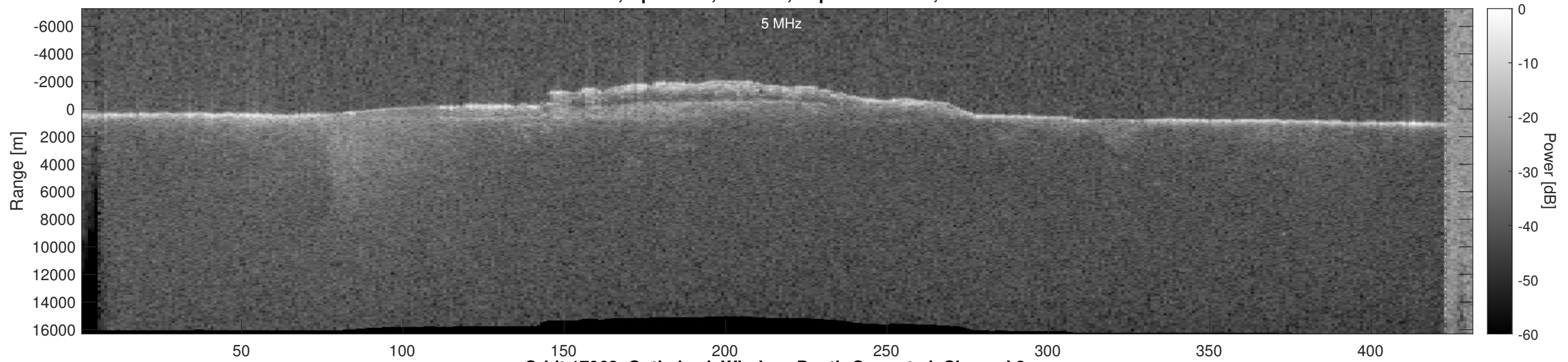
Orbit 17963, Optimized, Window, Depth-Corrected, Channel 2
