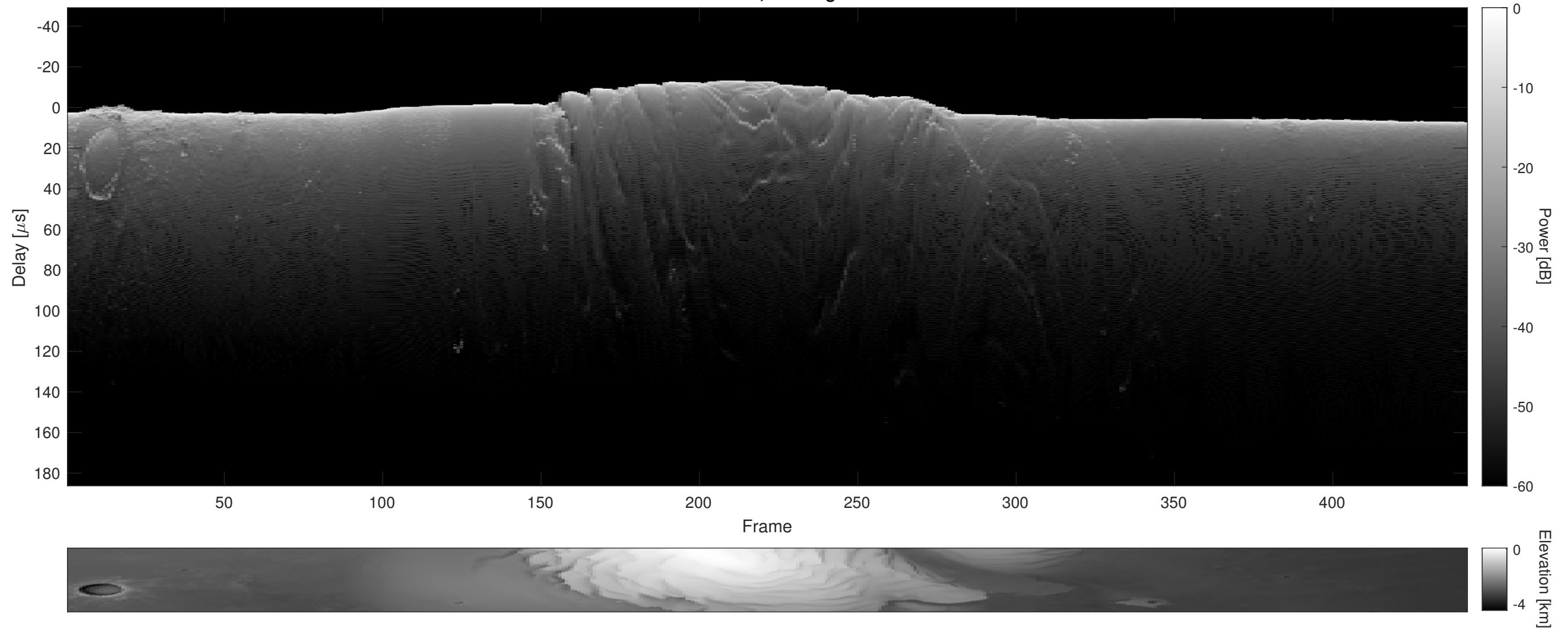
Orbit 17970, Cluttergram
