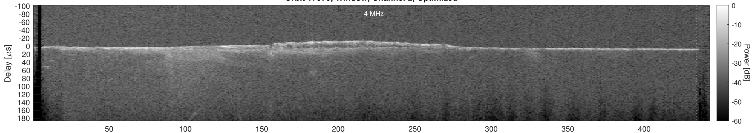
Orbit 17970, Cluttergram
