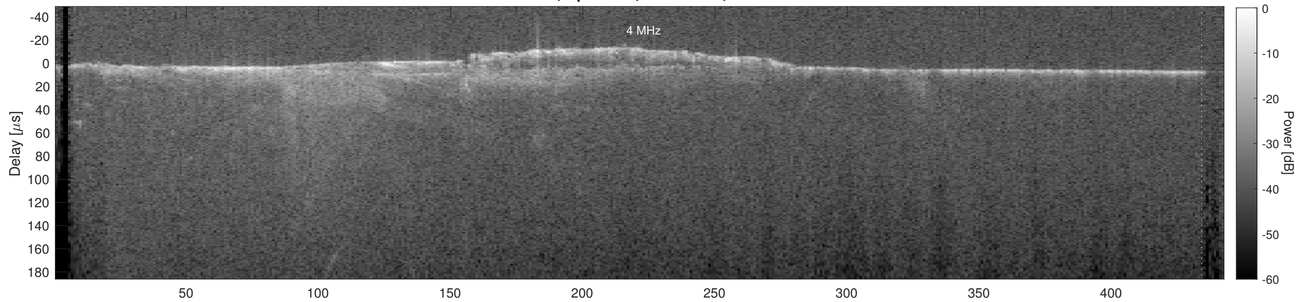
Orbit 17970, Cluttergram
