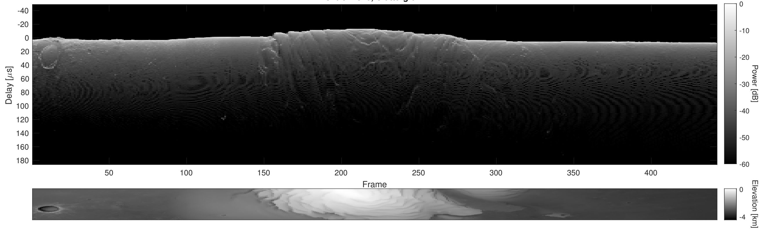
Orbit 17970, Cluttergram
