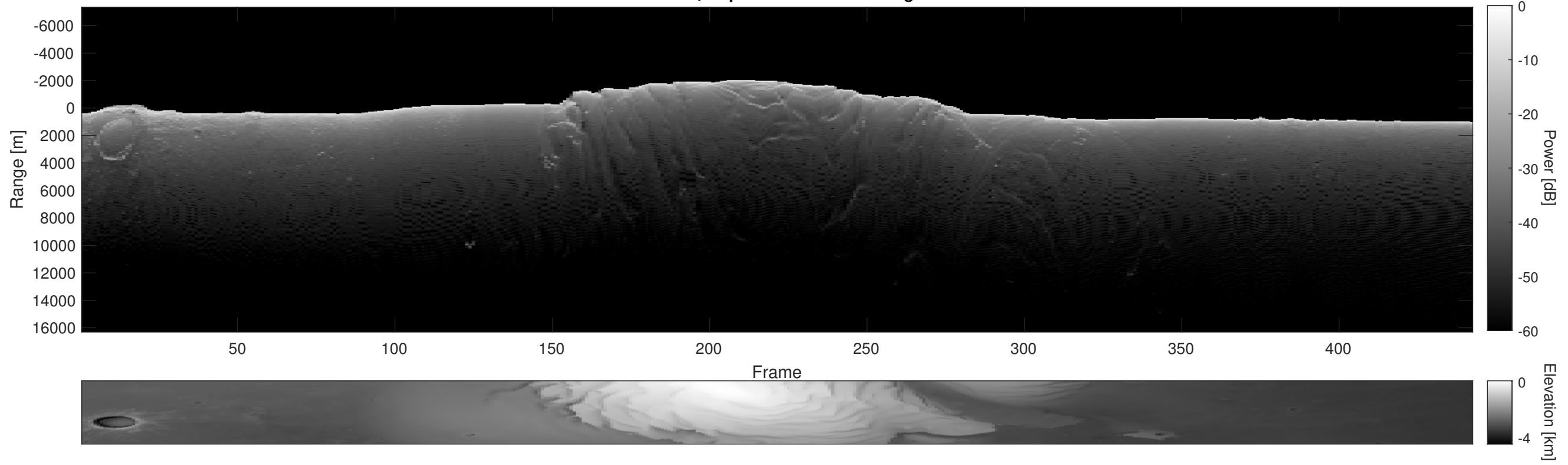
Orbit 17970, Depth-Corrected Cluttergram
