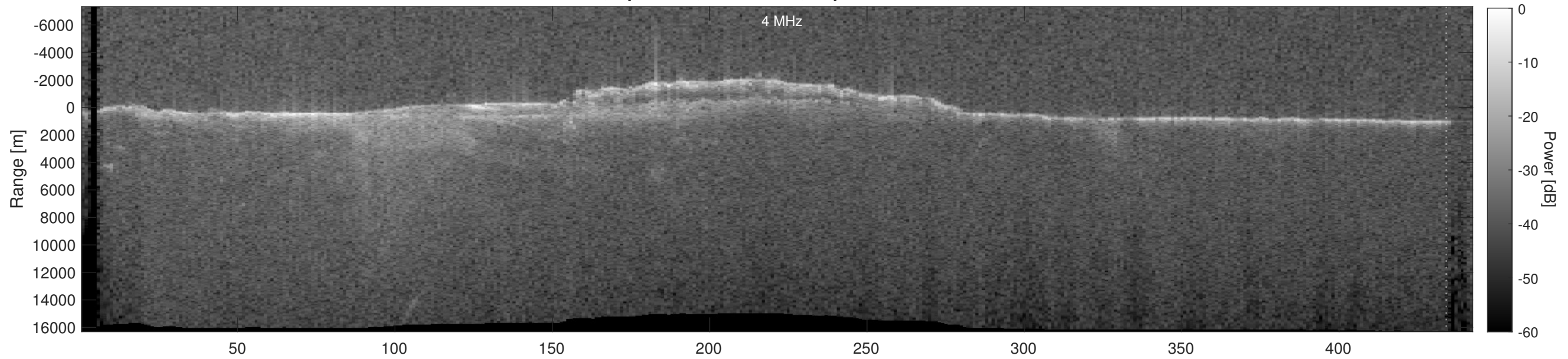
Orbit 17970, Depth-Corrected Cluttergram
