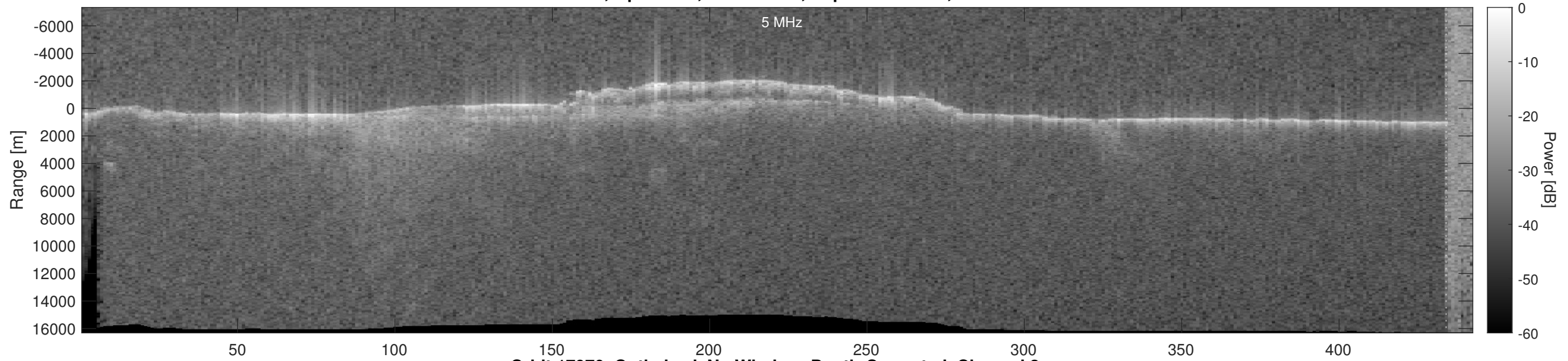
Orbit 17970, Optimized, No Window, Depth-Corrected, Channel 2
