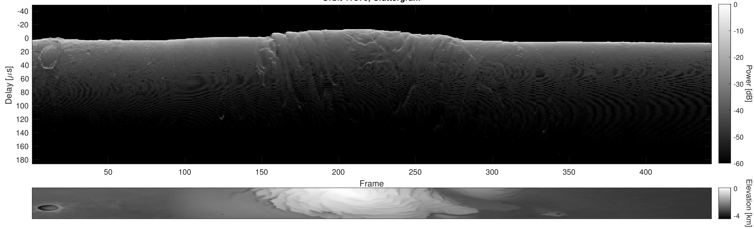
Orbit 17970, Cluttergram
