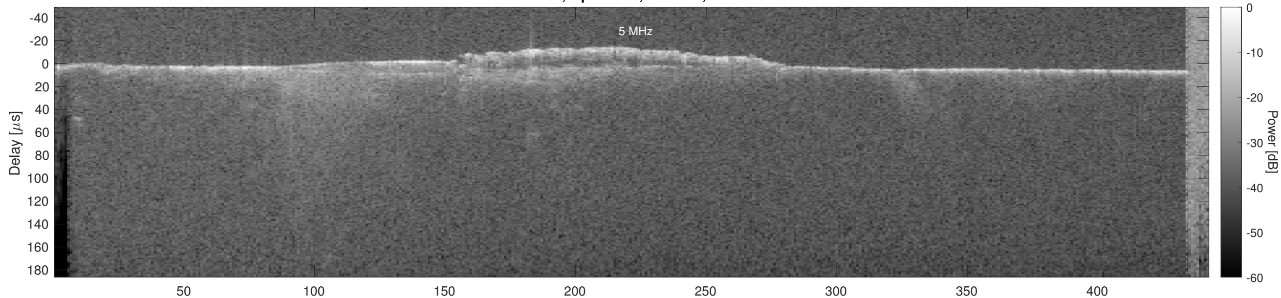
Orbit 17970, Optimized, Window, Channel 2
