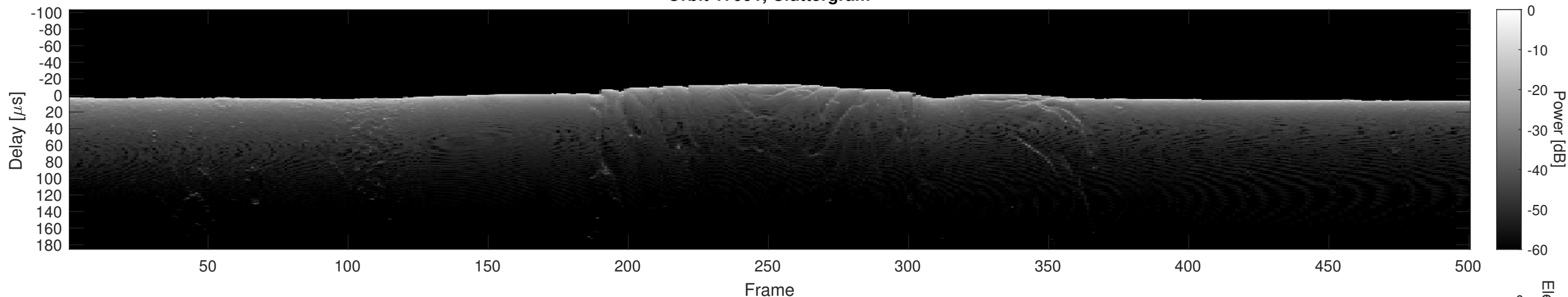
Orbit 17991, Cluttergram
