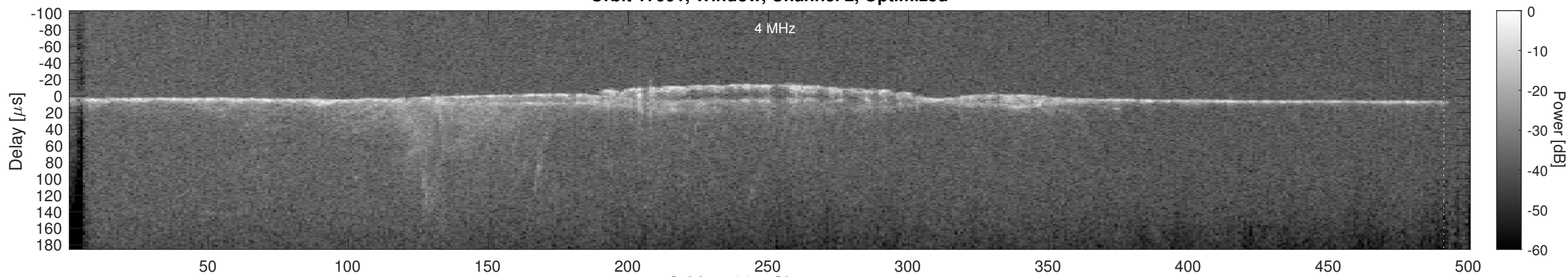
Orbit 17991, Cluttergram
