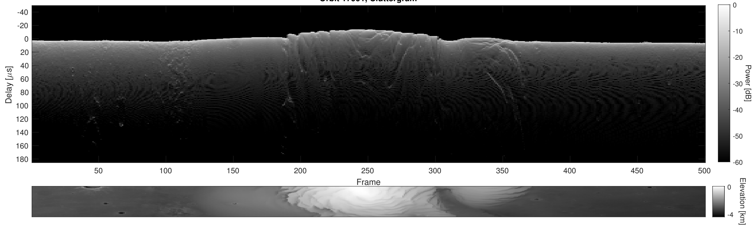
Orbit 17991, Cluttergram
