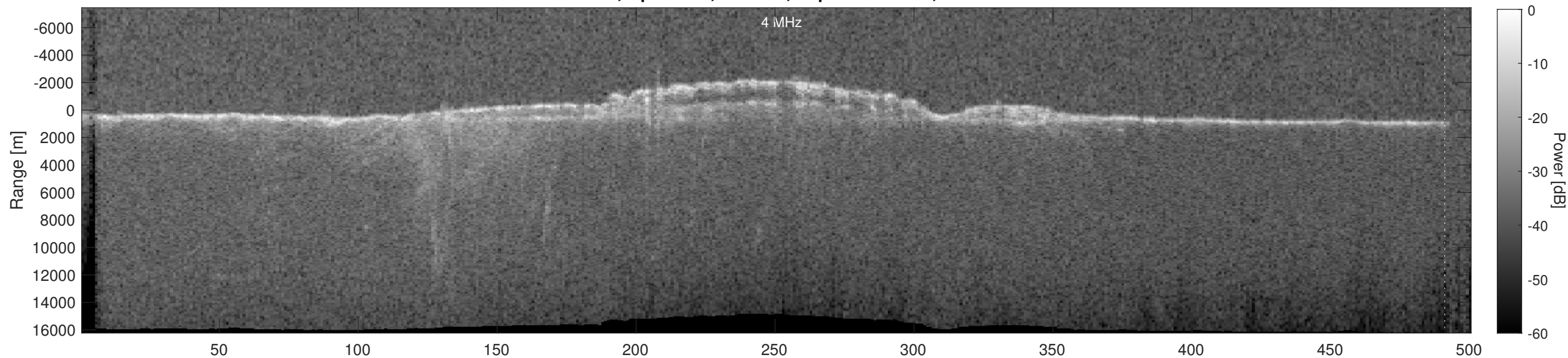
Orbit 17991, Depth-Corrected Cluttergram
