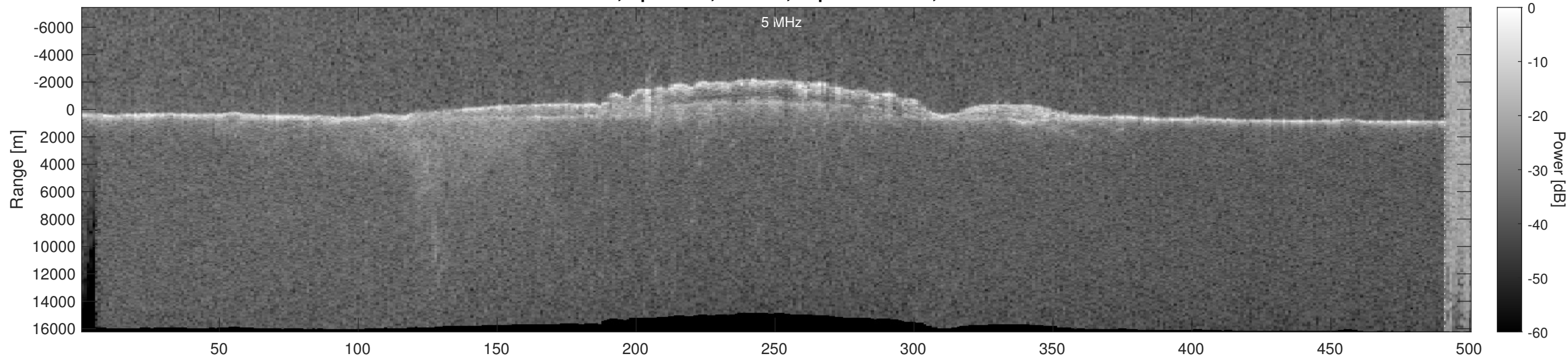
Orbit 17991, Optimized, Window, Depth-Corrected, Channel 2
