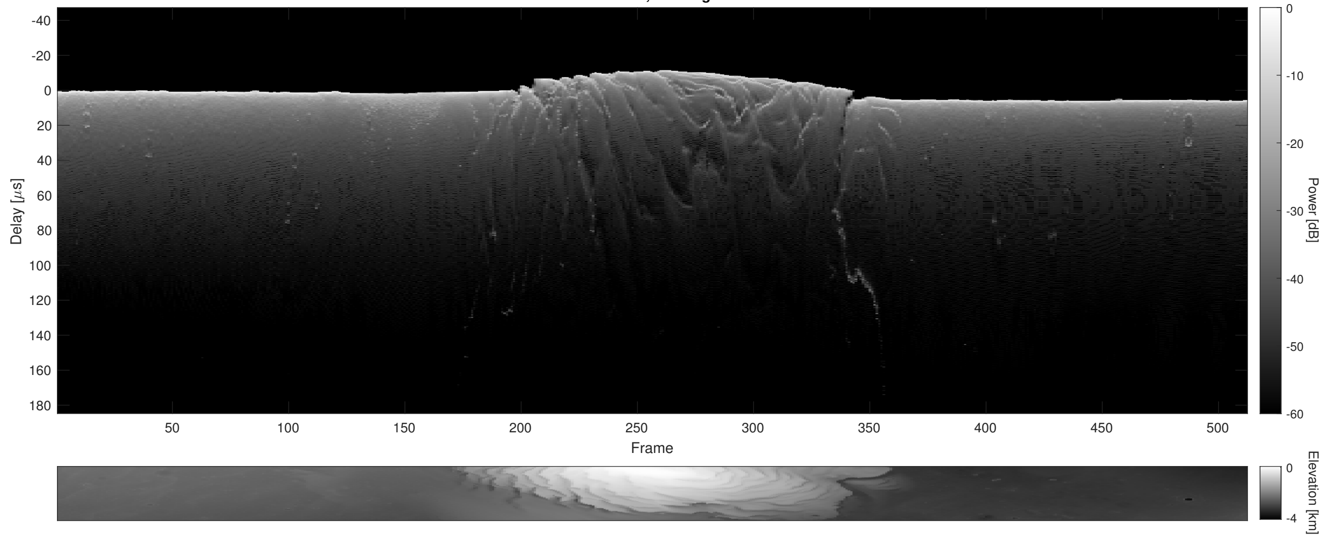
Orbit 17995, Cluttergram
