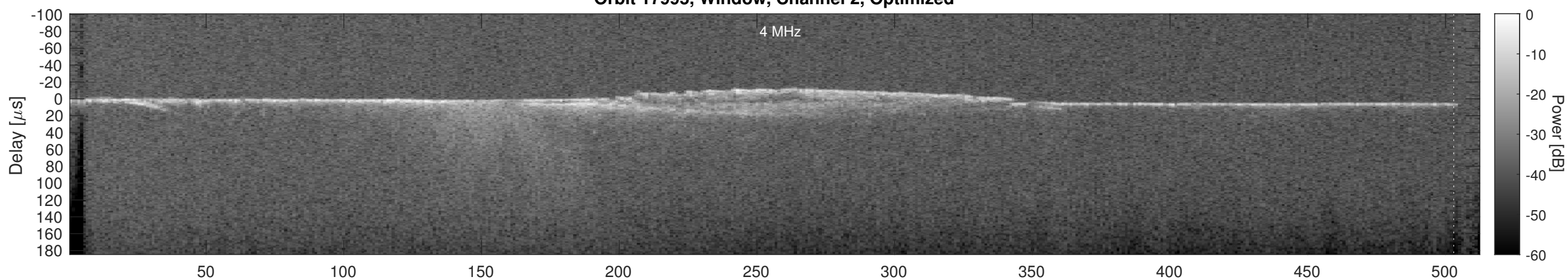
Orbit 17995, Cluttergram
