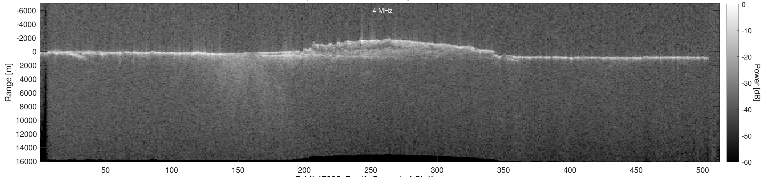
Orbit 17995, Depth-Corrected Cluttergram
