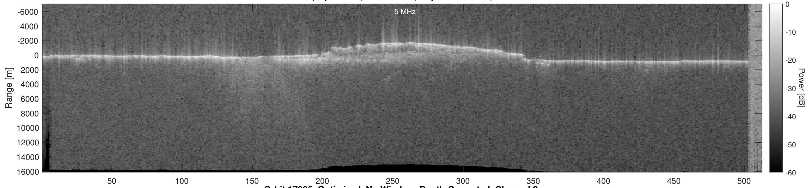
Orbit 17995, Optimized, No Window, Depth-Corrected, Channel 2
