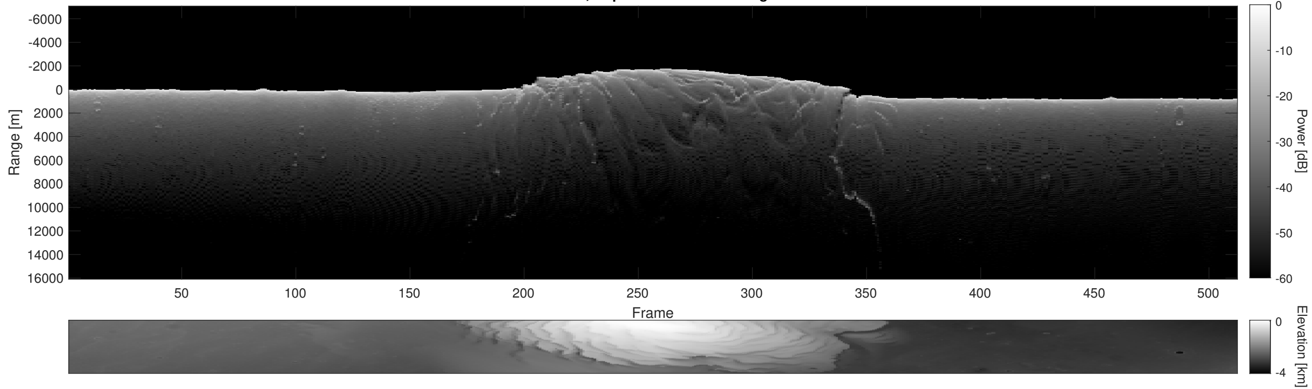
Orbit 17995, Depth-Corrected Cluttergram
