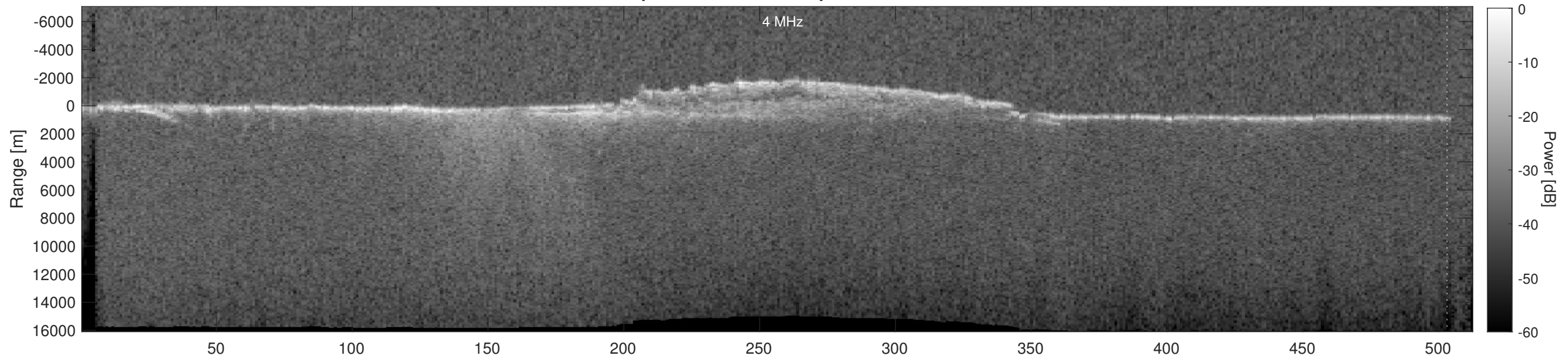
Orbit 17995, Depth-Corrected Cluttergram
