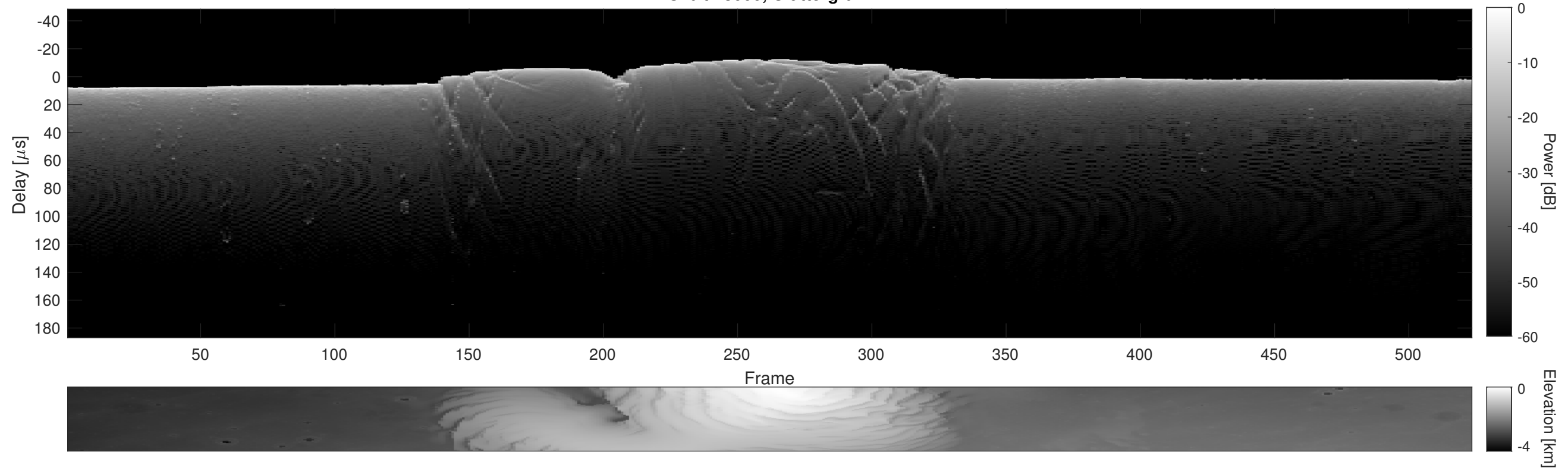
Orbit 18000, Cluttergram
