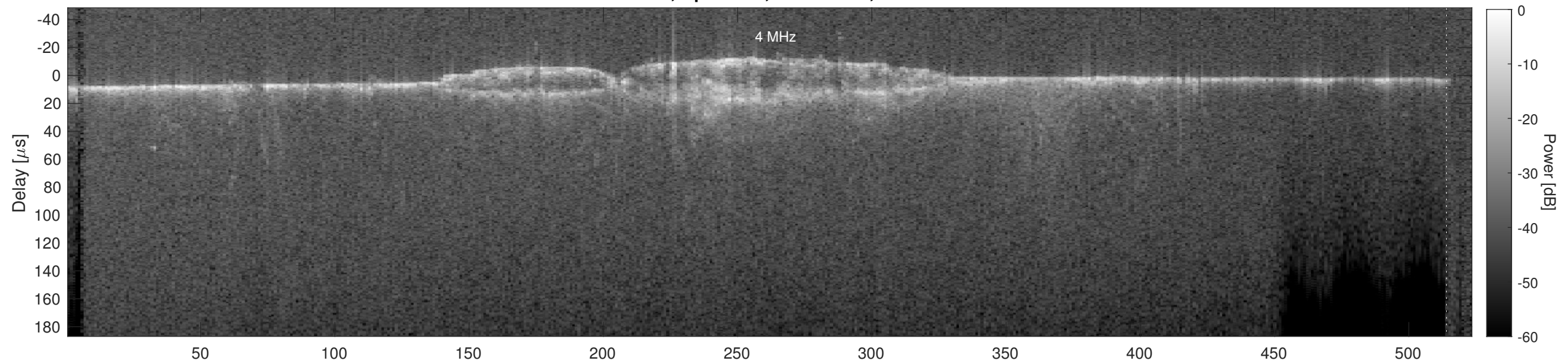
Orbit 18000, Cluttergram
