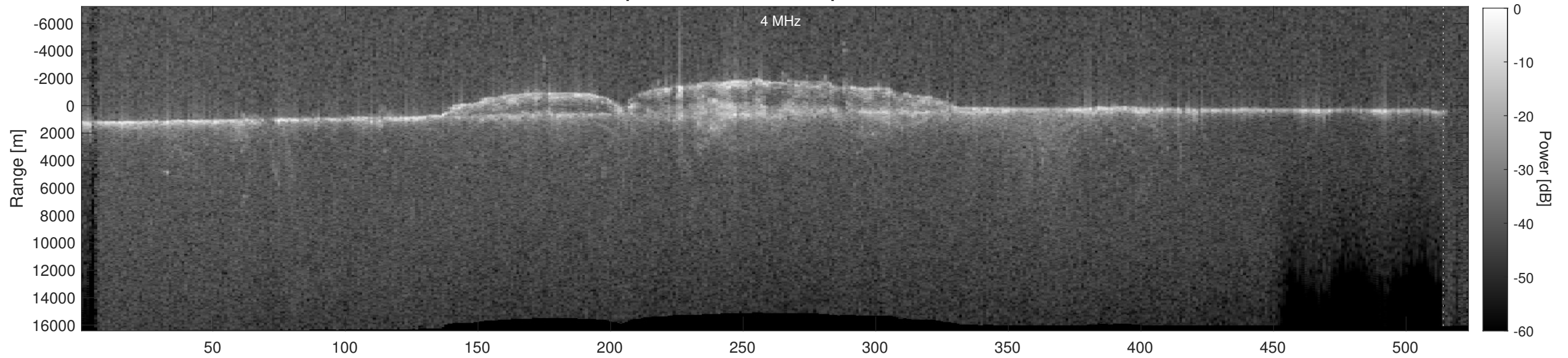
Orbit 18000, Depth-Corrected Cluttergram
