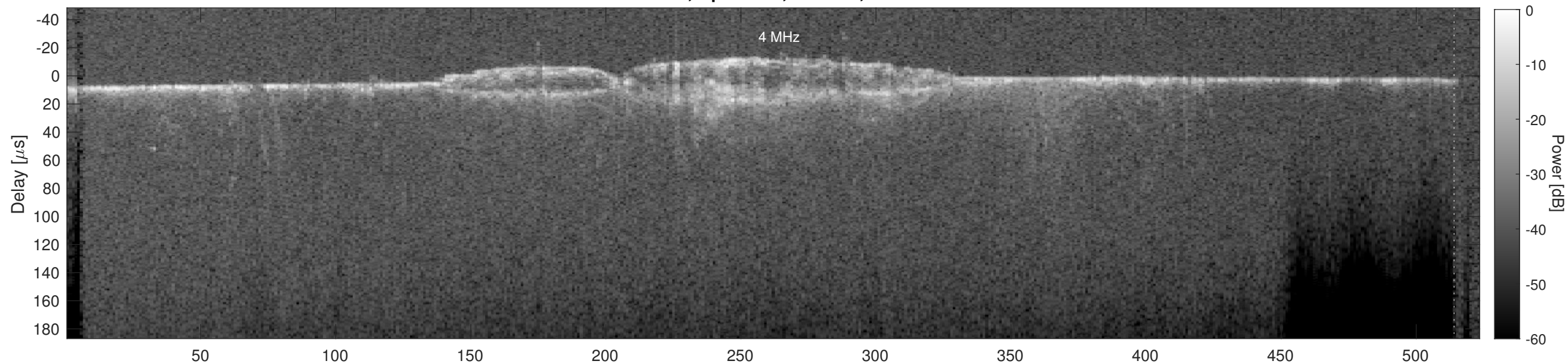
Orbit 18000, Cluttergram
