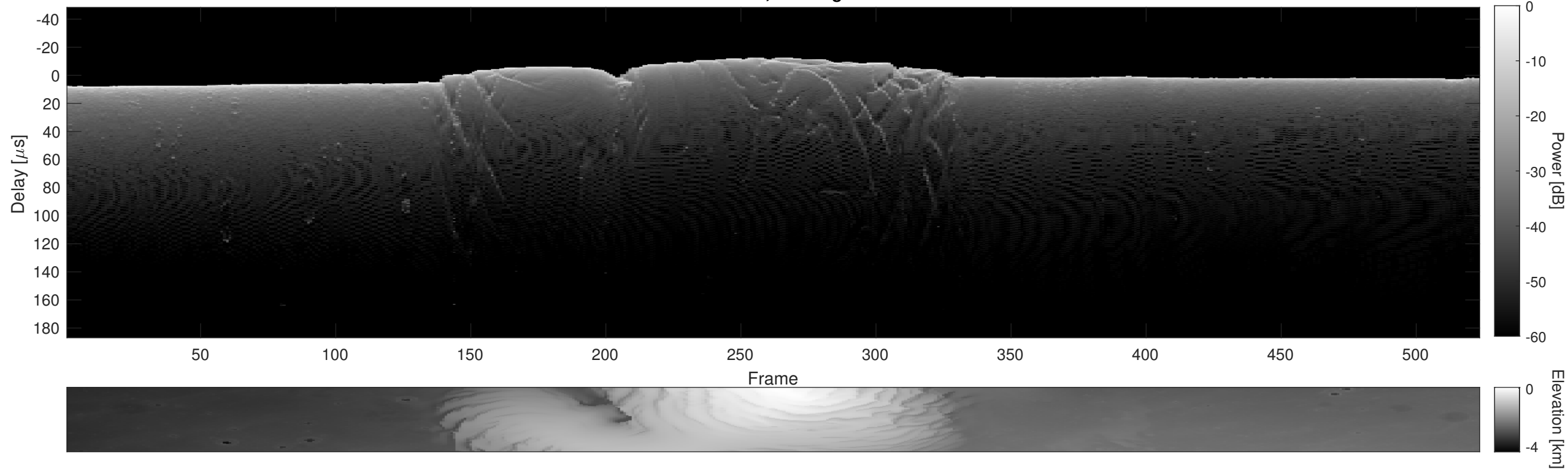
Orbit 18000, Cluttergram
