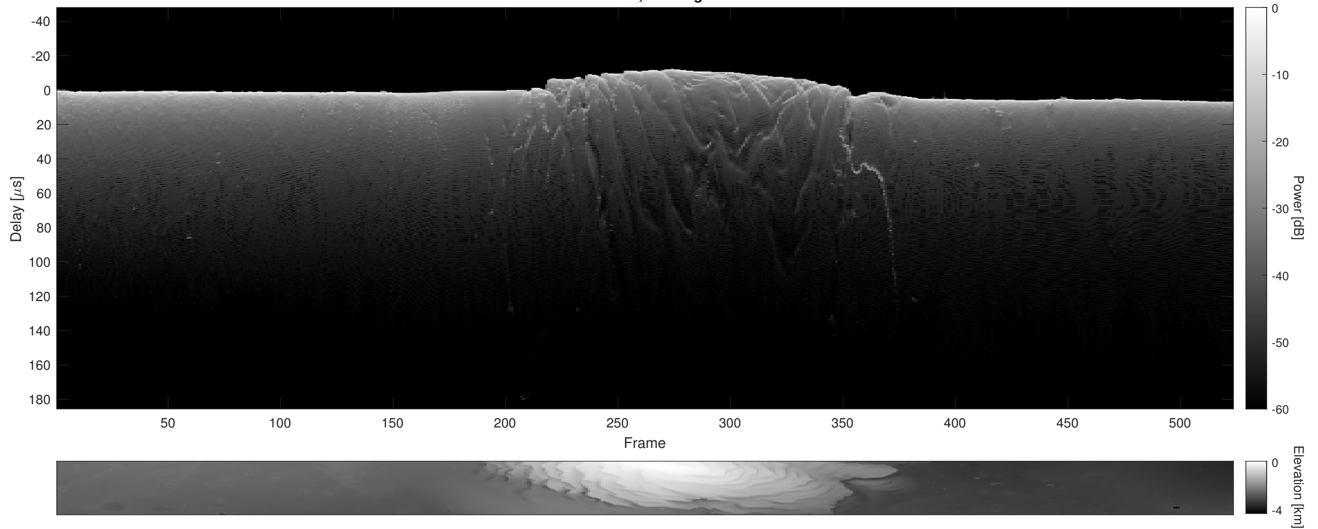
Orbit 18002, Cluttergram
