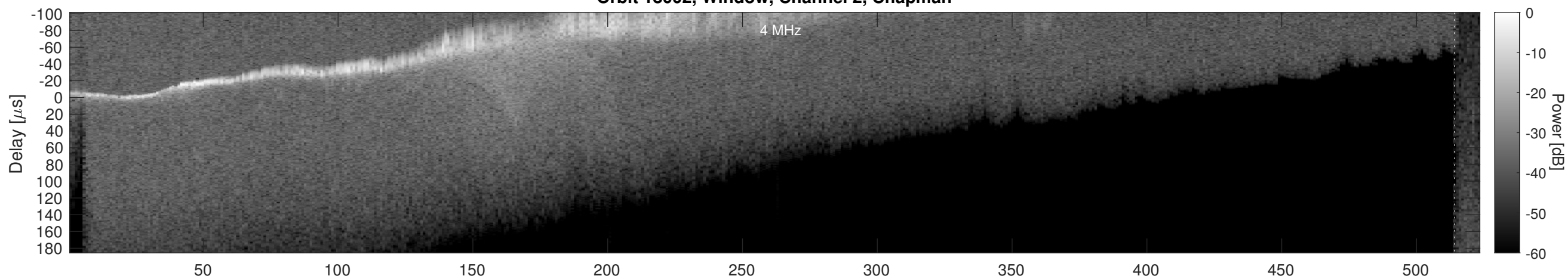
Orbit 18002, Window, Channel 2, Optimized
