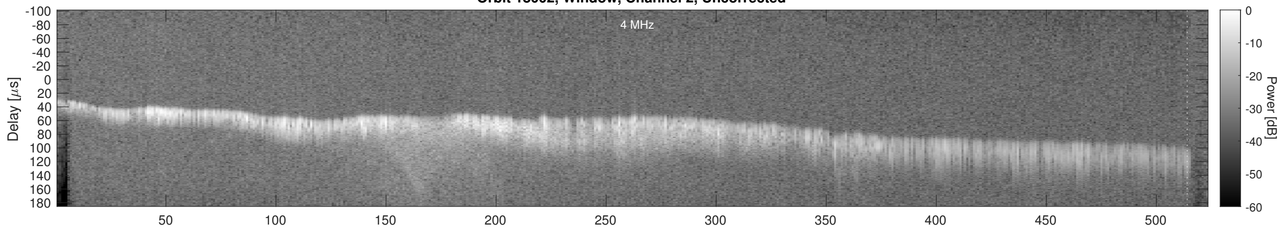
Orbit 18002, Window, Channel 2, Chapman
