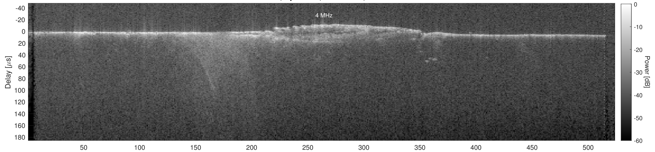
Orbit 18002, Cluttergram
