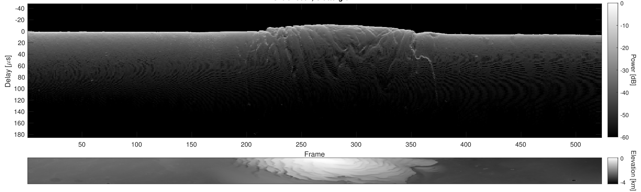
Orbit 18002, Cluttergram
