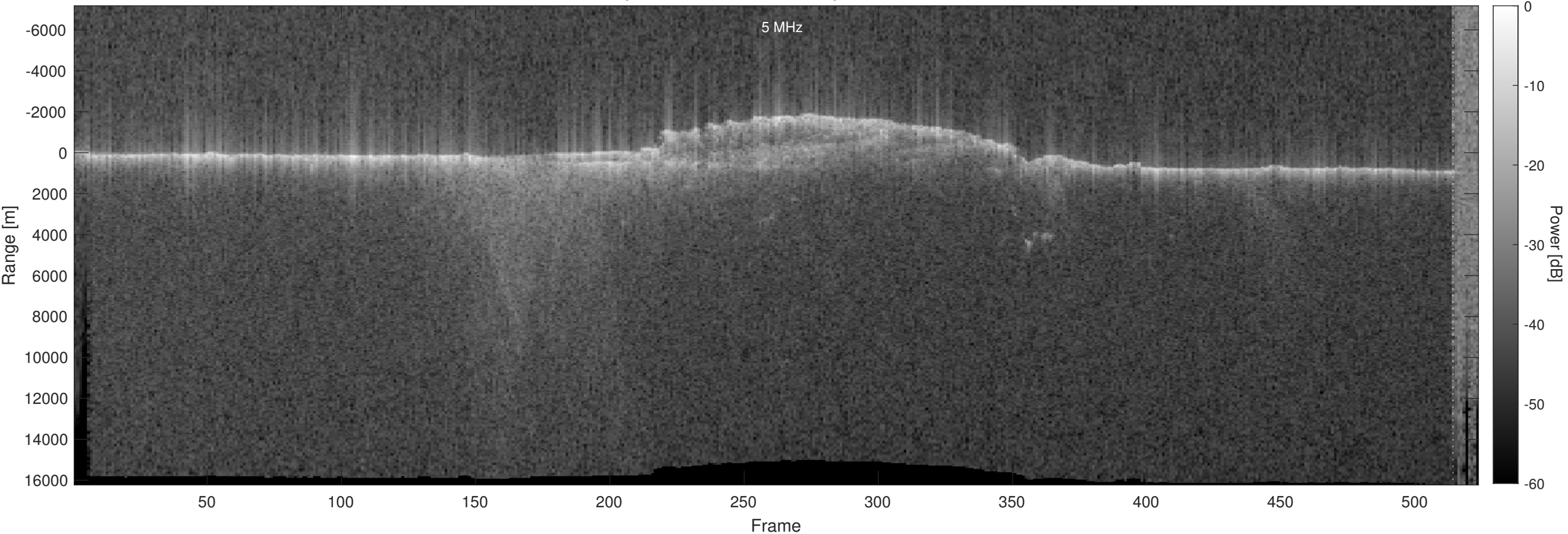
Orbit 18002, Optimized, No Window, Depth-Corrected, Channel 2
