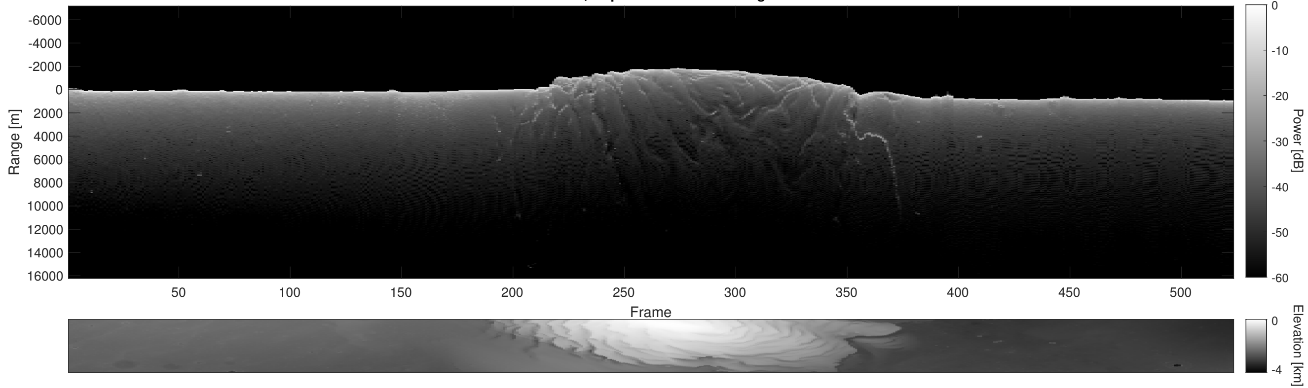
Orbit 18002, Depth-Corrected Cluttergram
