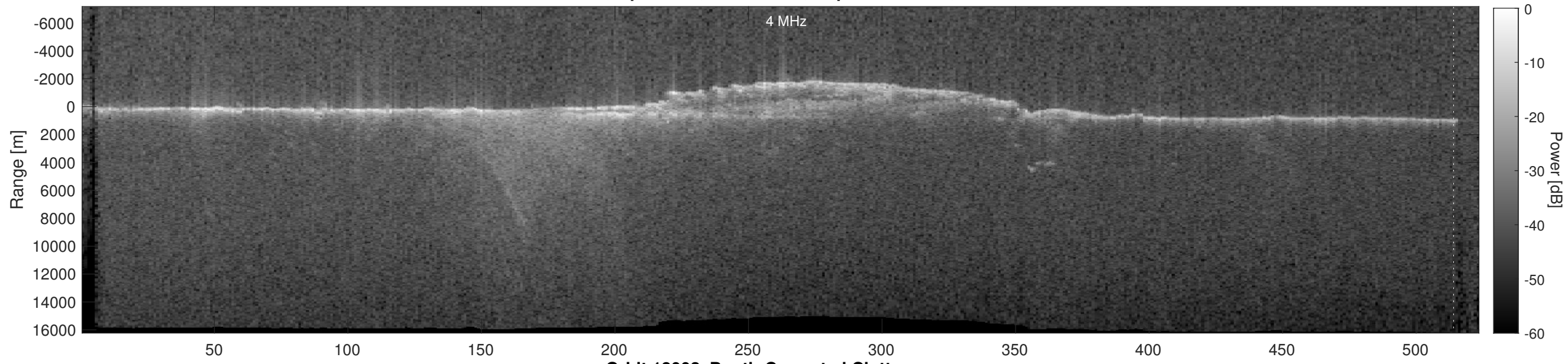
Orbit 18002, Depth-Corrected Cluttergram
