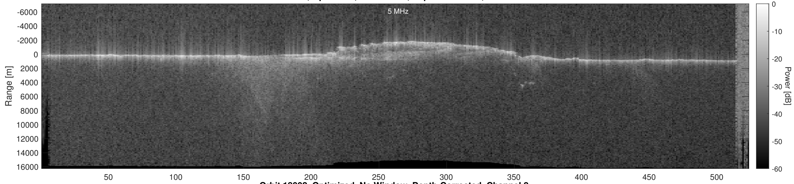
Orbit 18002, Optimized, No Window, Depth-Corrected, Channel 2
