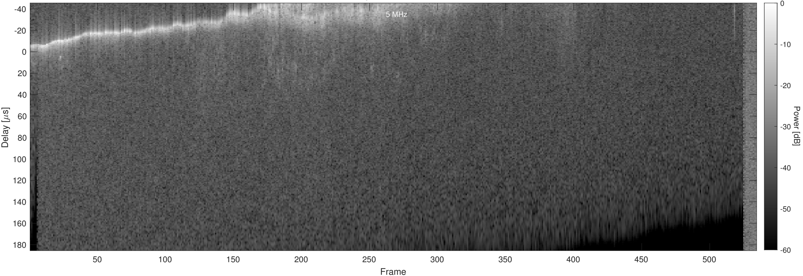
Orbit 18006, Chapman, No Window, Channel 2
