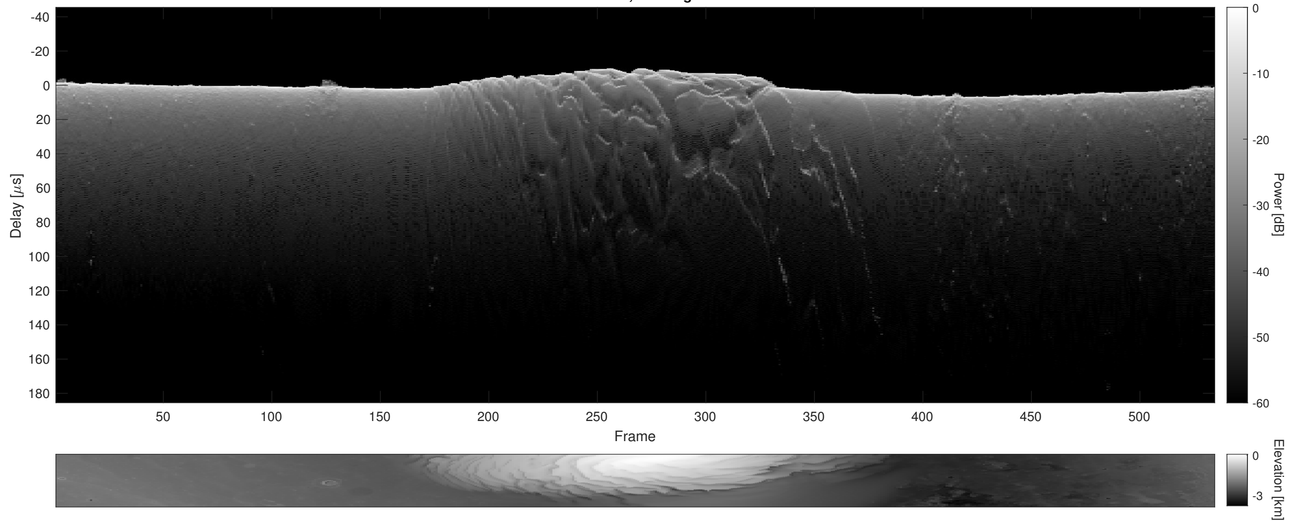
Orbit 18006, Cluttergram
