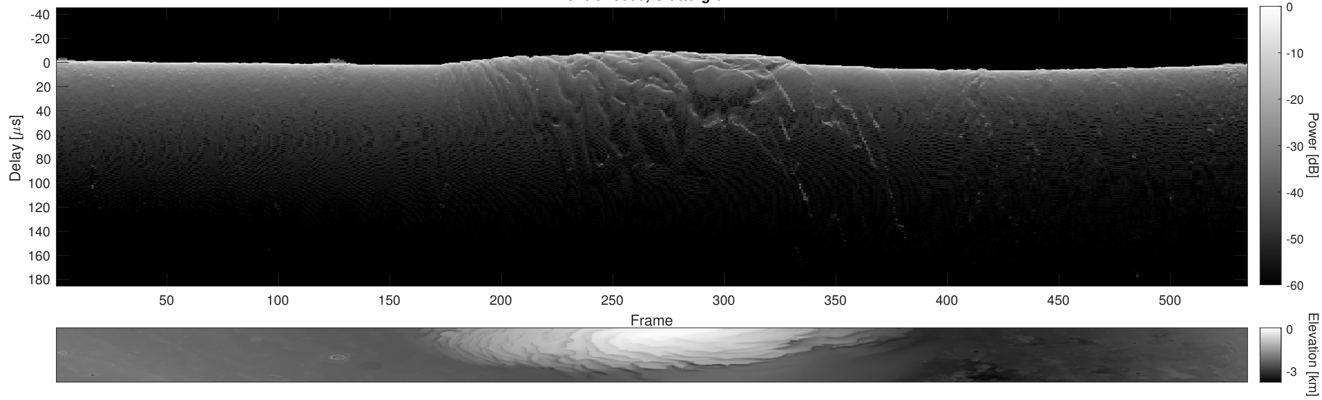
Orbit 18006, Cluttergram
