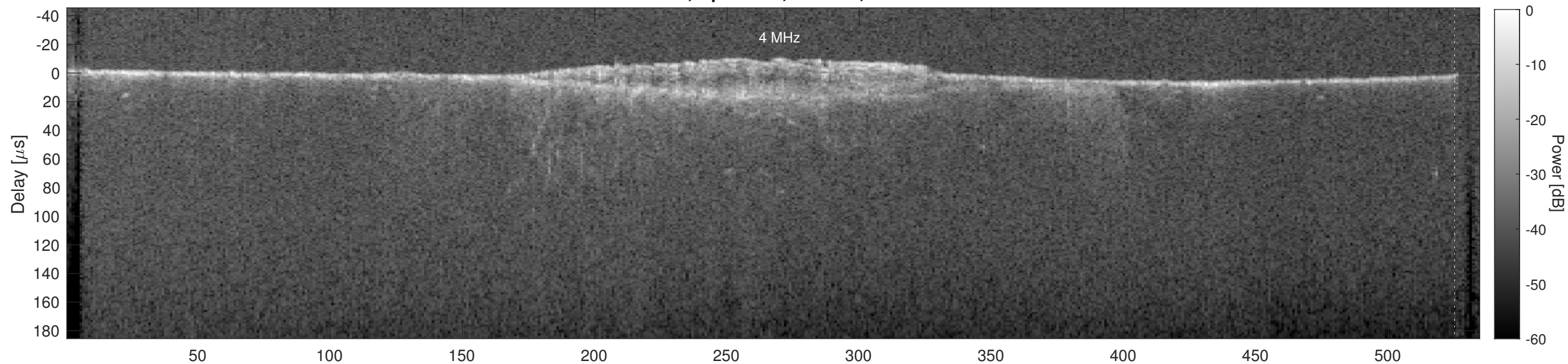
Orbit 18006, Cluttergram
