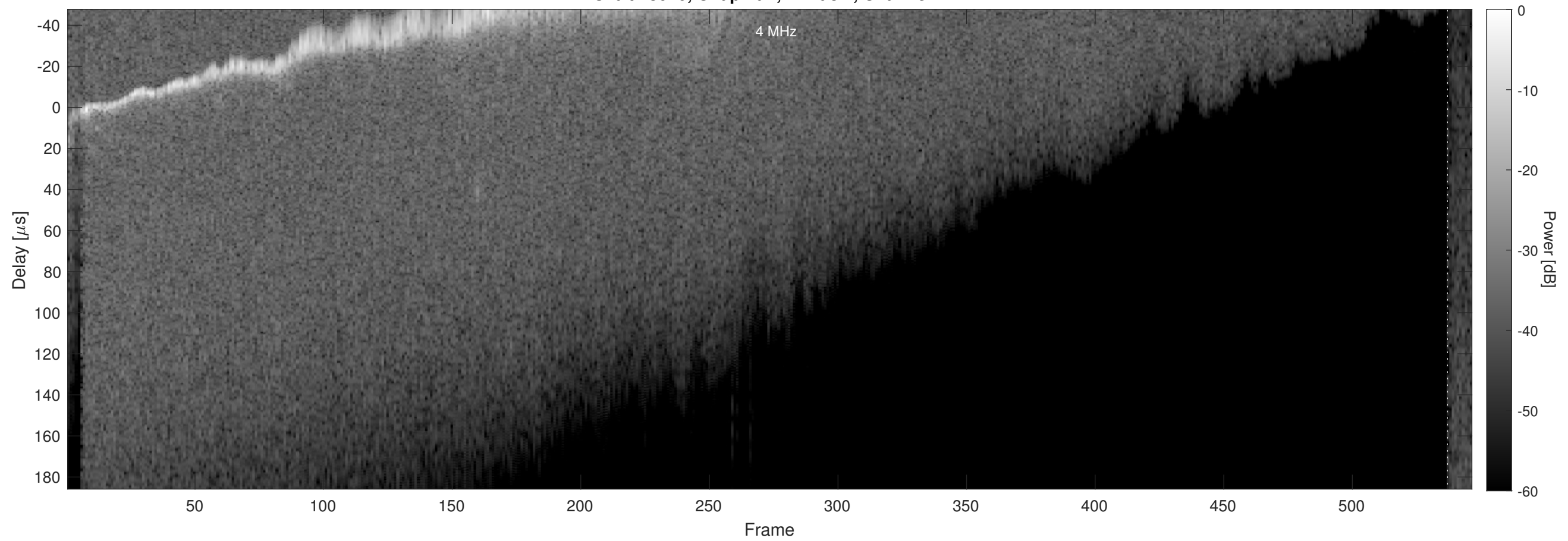
Orbit 18010, Chapman, Window, Channel 2
