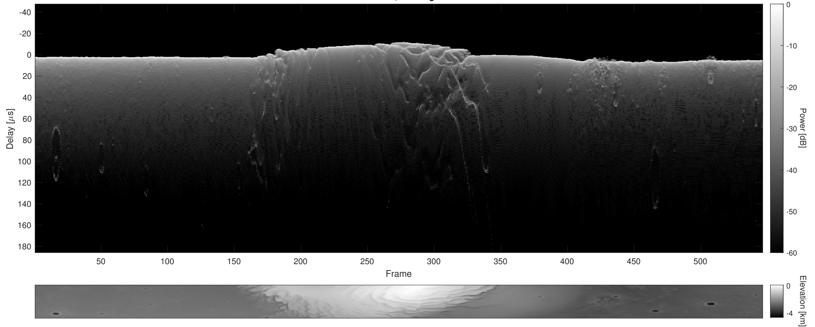
Orbit 18010, Cluttergram
