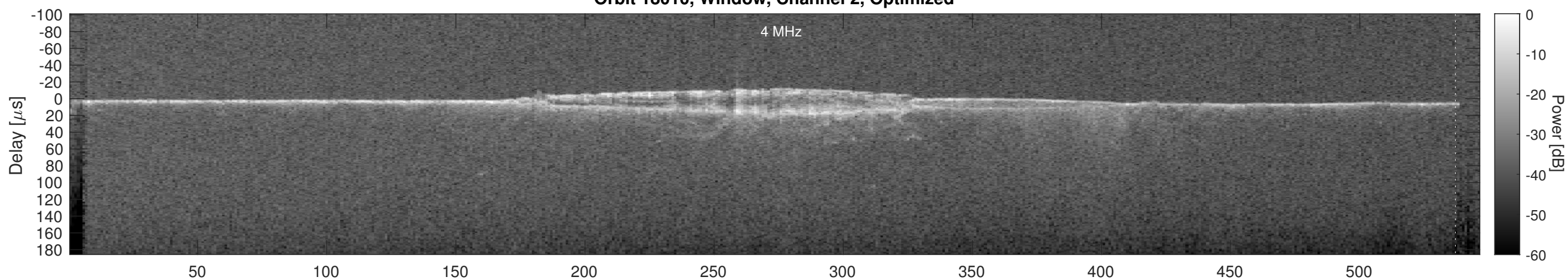
Orbit 18010, Cluttergram
