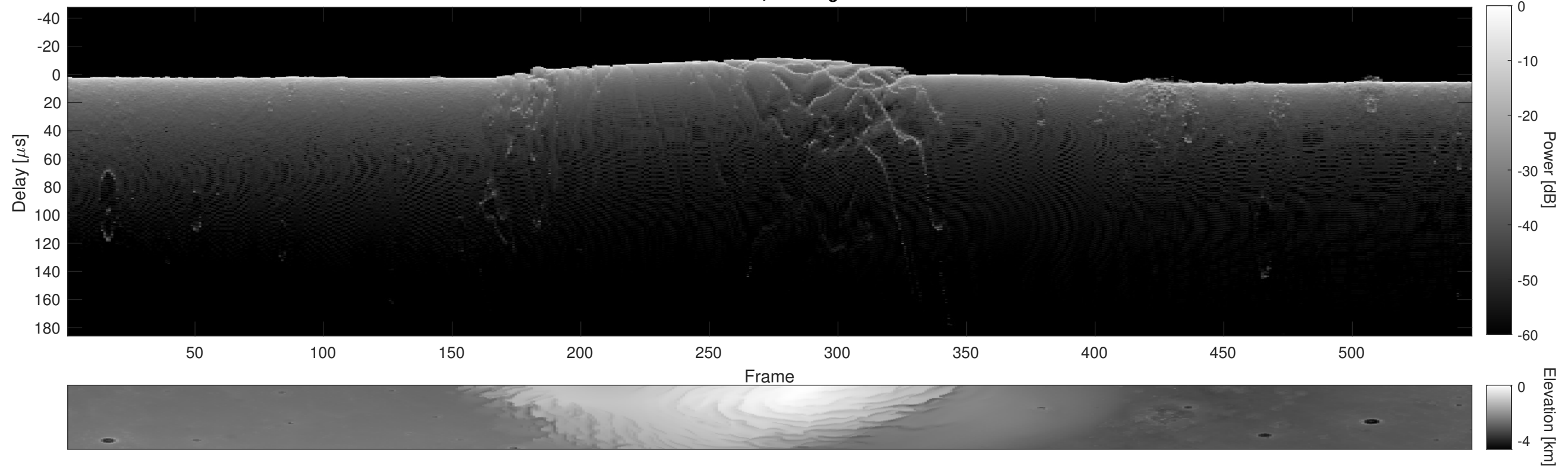
Orbit 18010, Cluttergram
