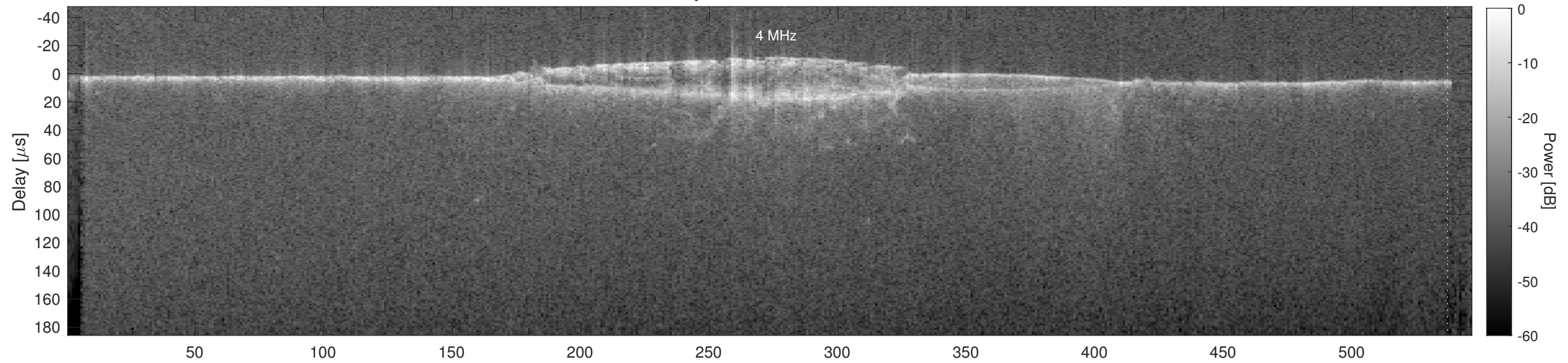
Orbit 18010, Cluttergram
