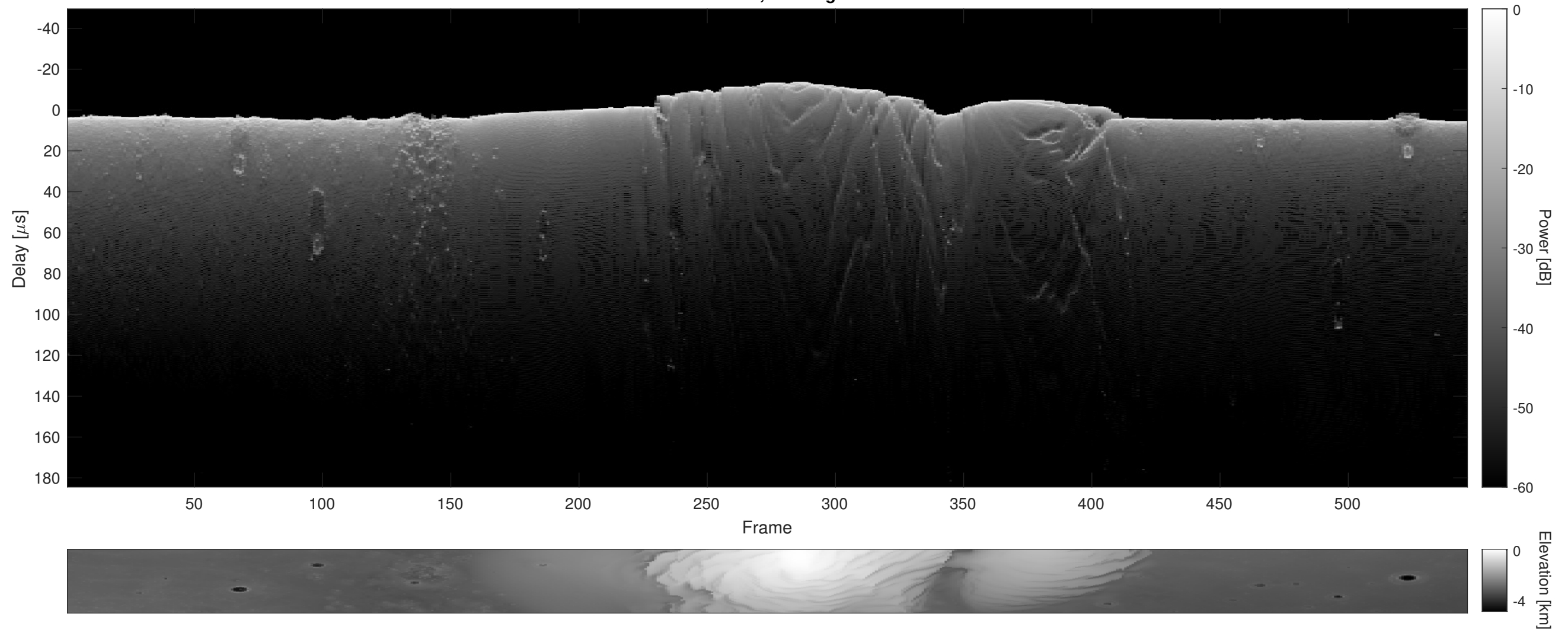
Orbit 18012, Cluttergram
