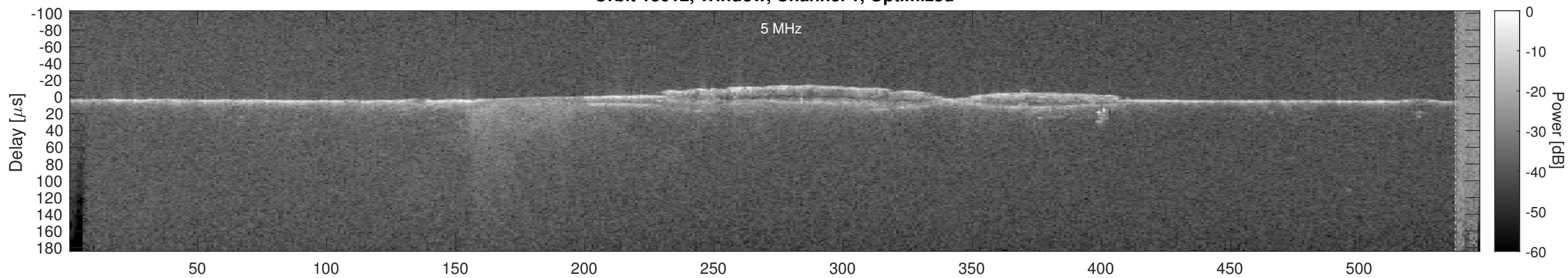
Orbit 18012, Cluttergram
