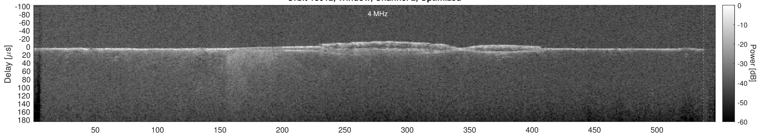
Orbit 18012, Cluttergram
