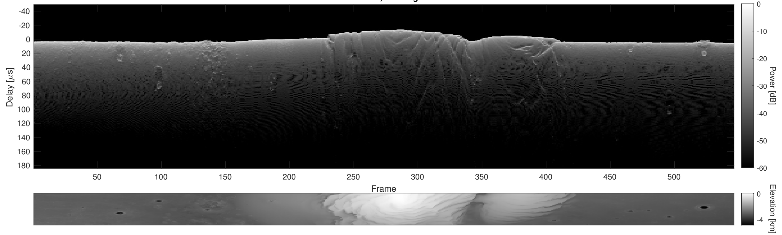
Orbit 18012, Cluttergram
