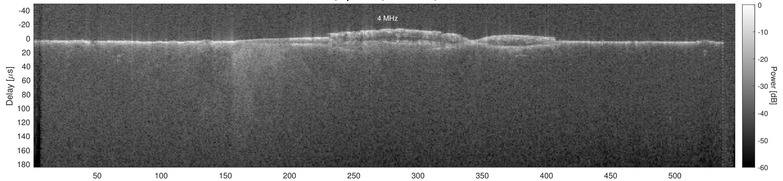
Orbit 18012, Cluttergram
