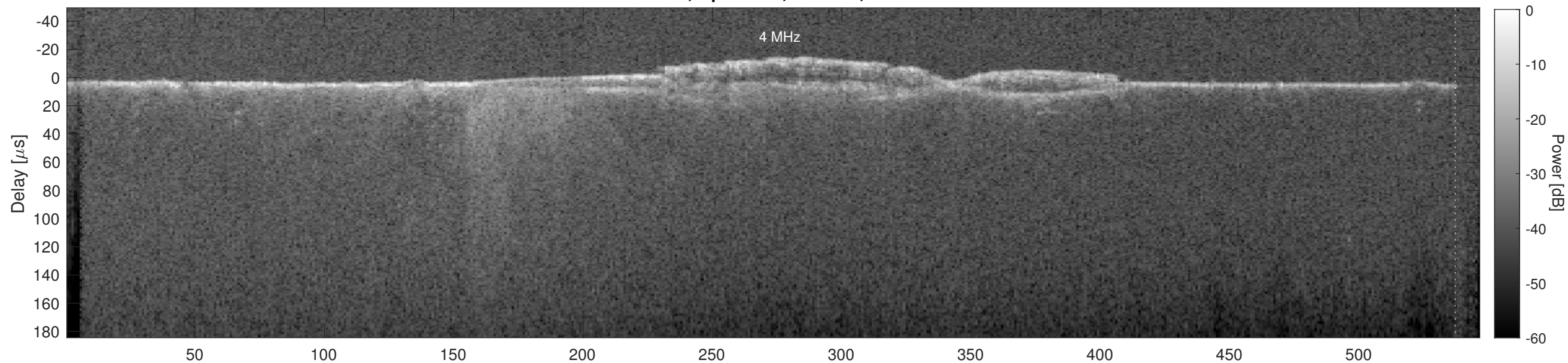
Orbit 18012, Cluttergram
