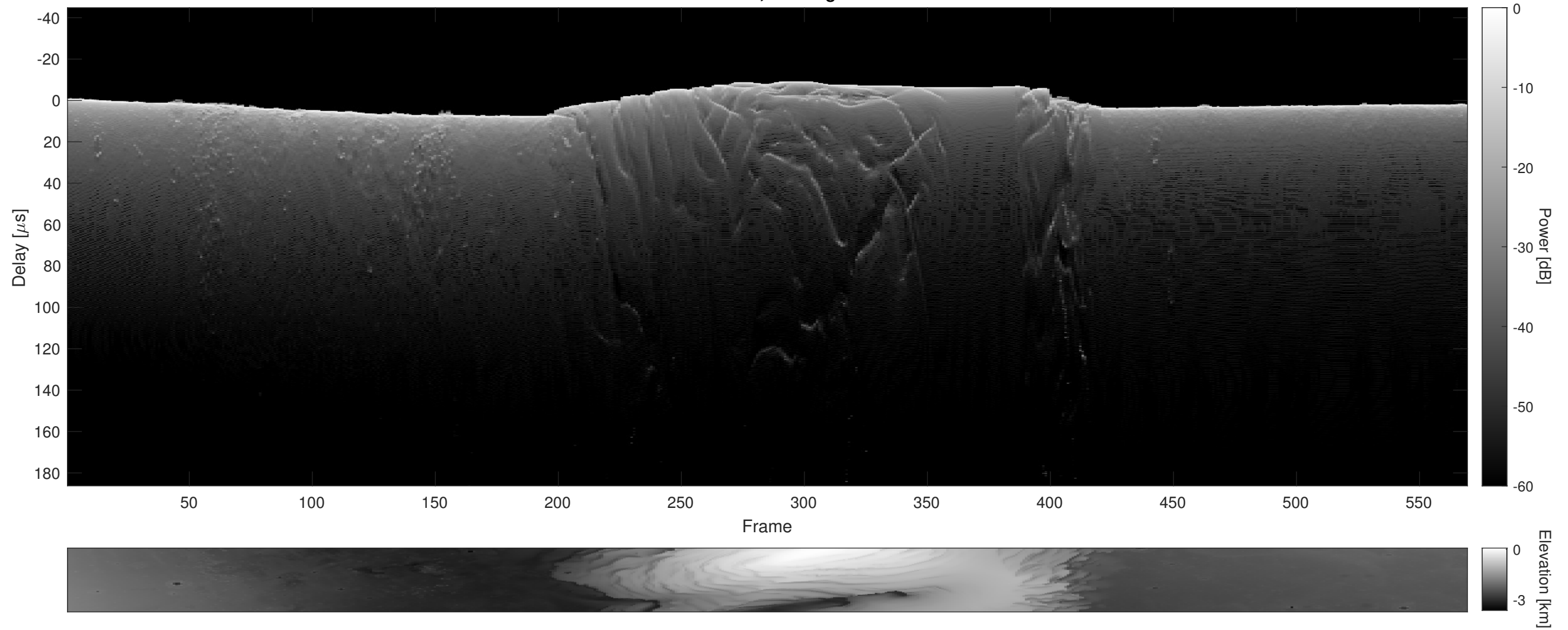
Orbit 18022, Cluttergram
