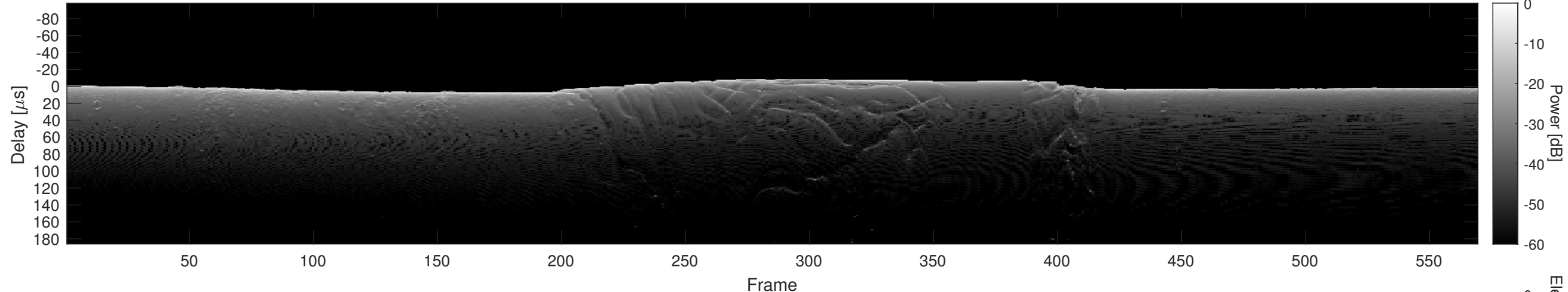
Orbit 18022, Cluttergram
