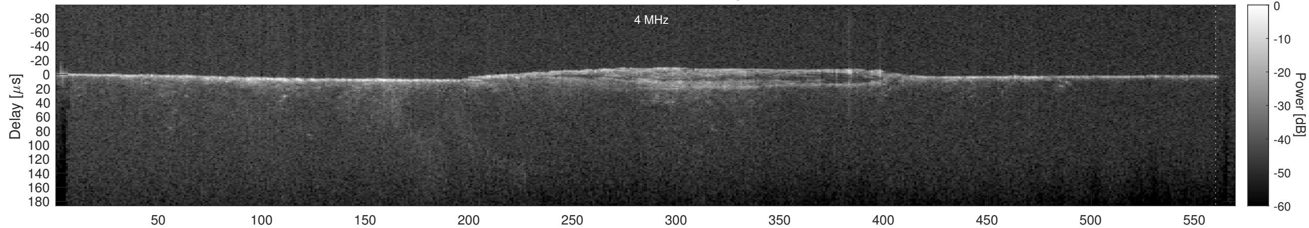
Orbit 18022, Cluttergram
