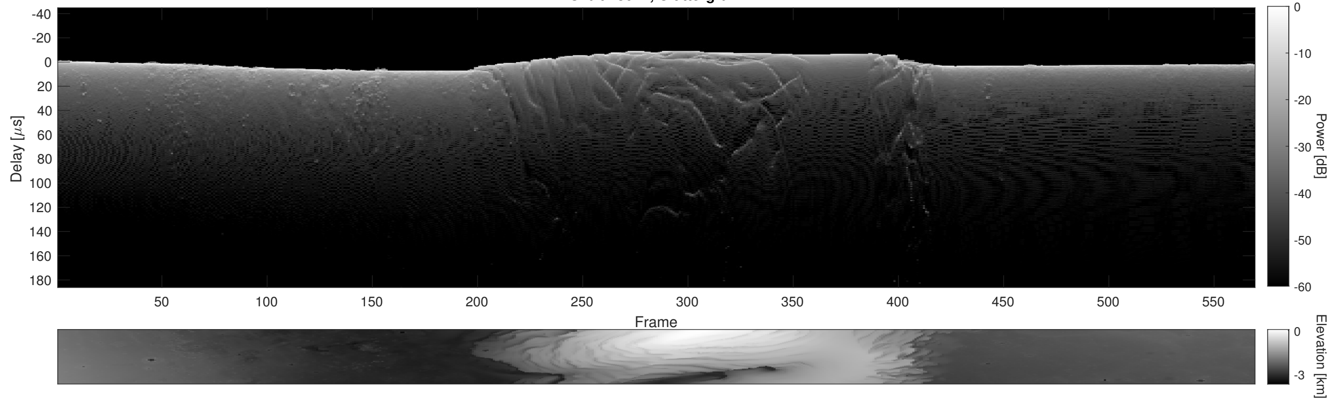
Orbit 18022, Cluttergram
