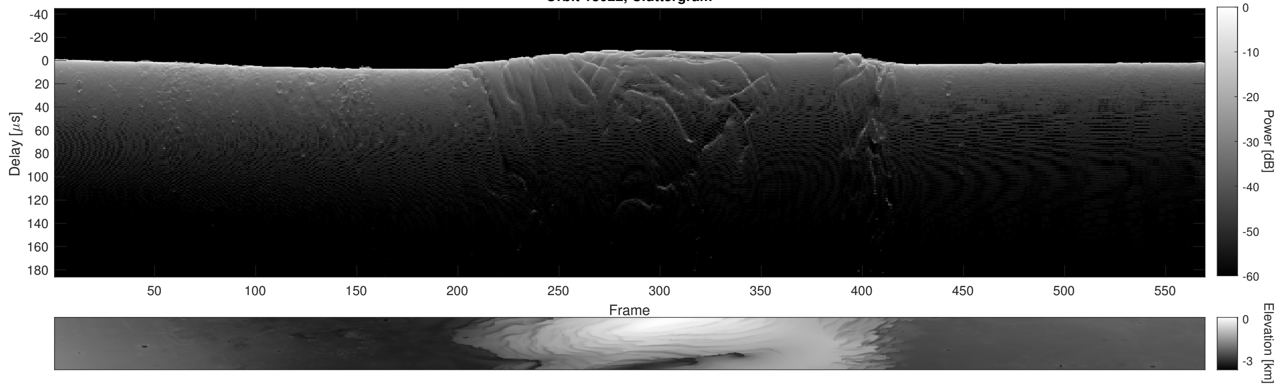
Orbit 18022, Cluttergram
