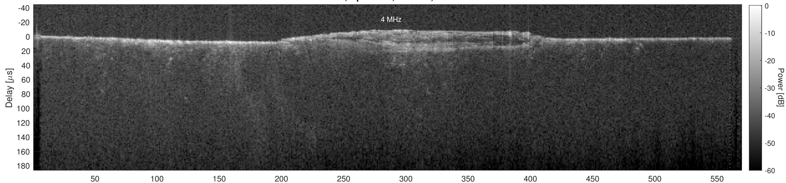
Orbit 18022, Cluttergram
