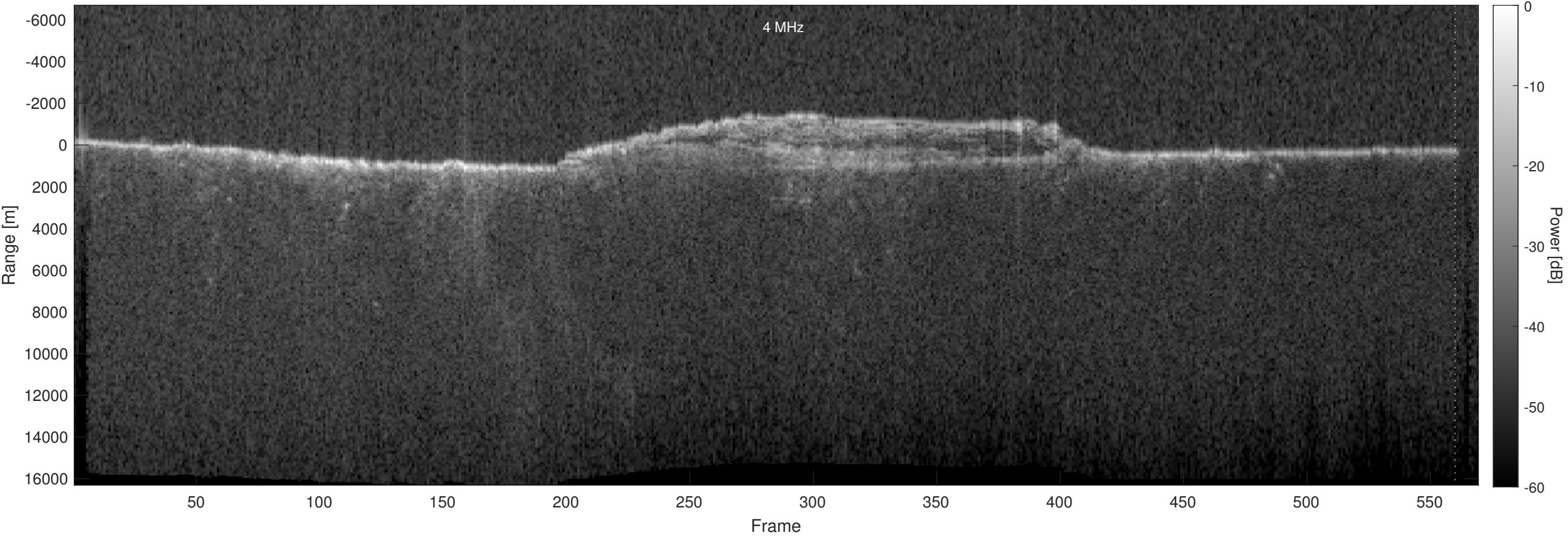
Orbit 18022, Optimized, Window, Depth-Corrected, Channel 2
