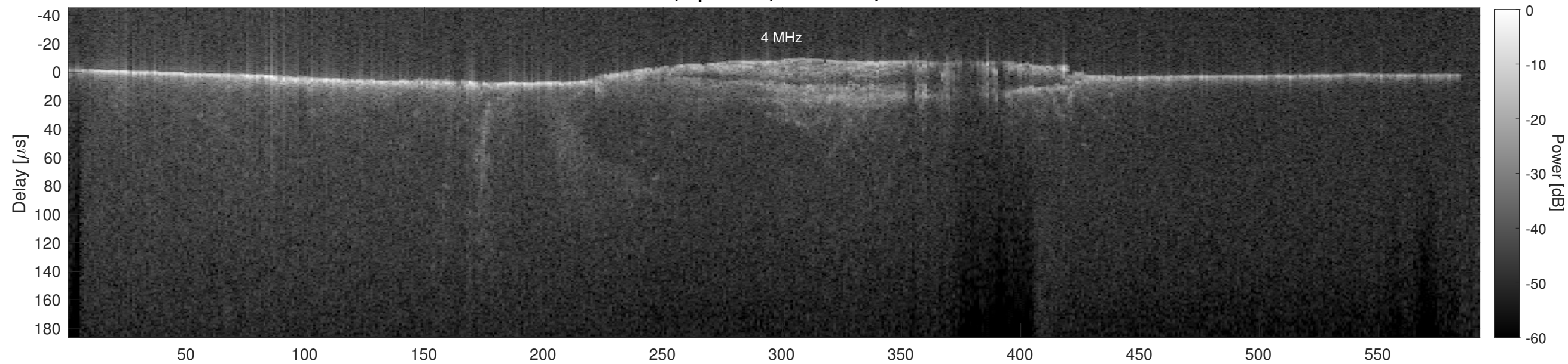
Orbit 18029, Cluttergram
