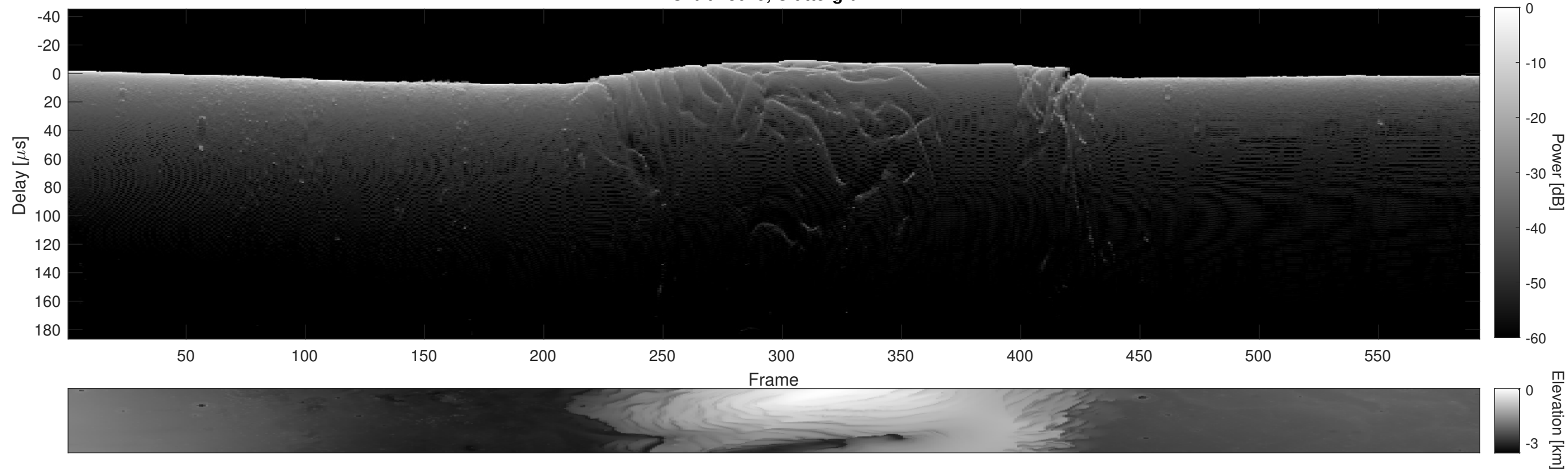
Orbit 18029, Cluttergram
