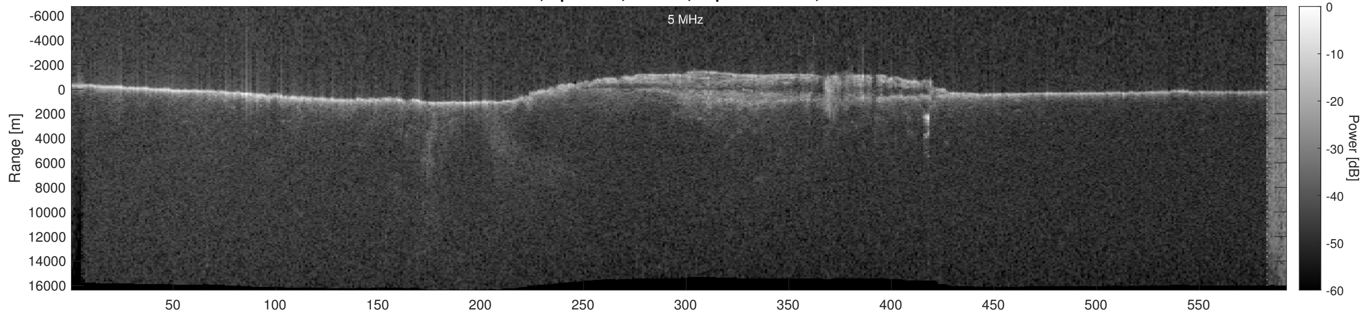
Orbit 18029, Optimized, Window, Depth-Corrected, Channel 2
