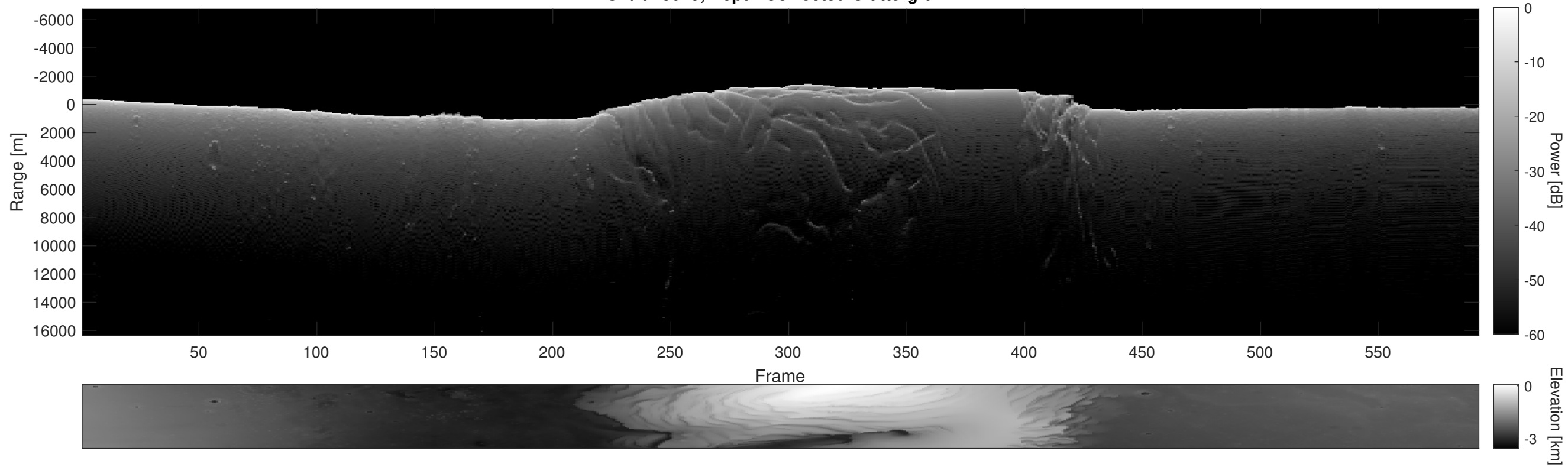
Orbit 18029, Depth-Corrected Cluttergram
