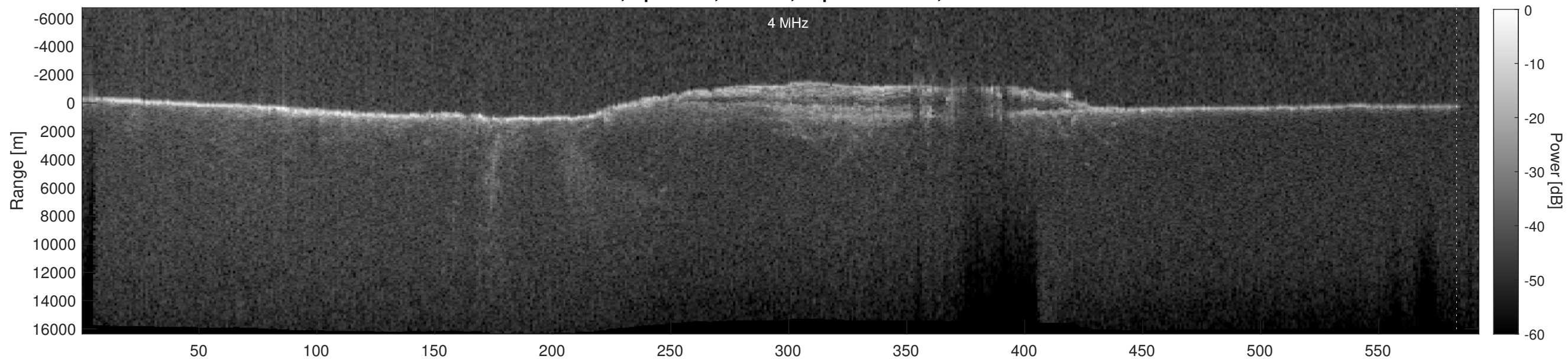
Orbit 18029, Depth-Corrected Cluttergram
