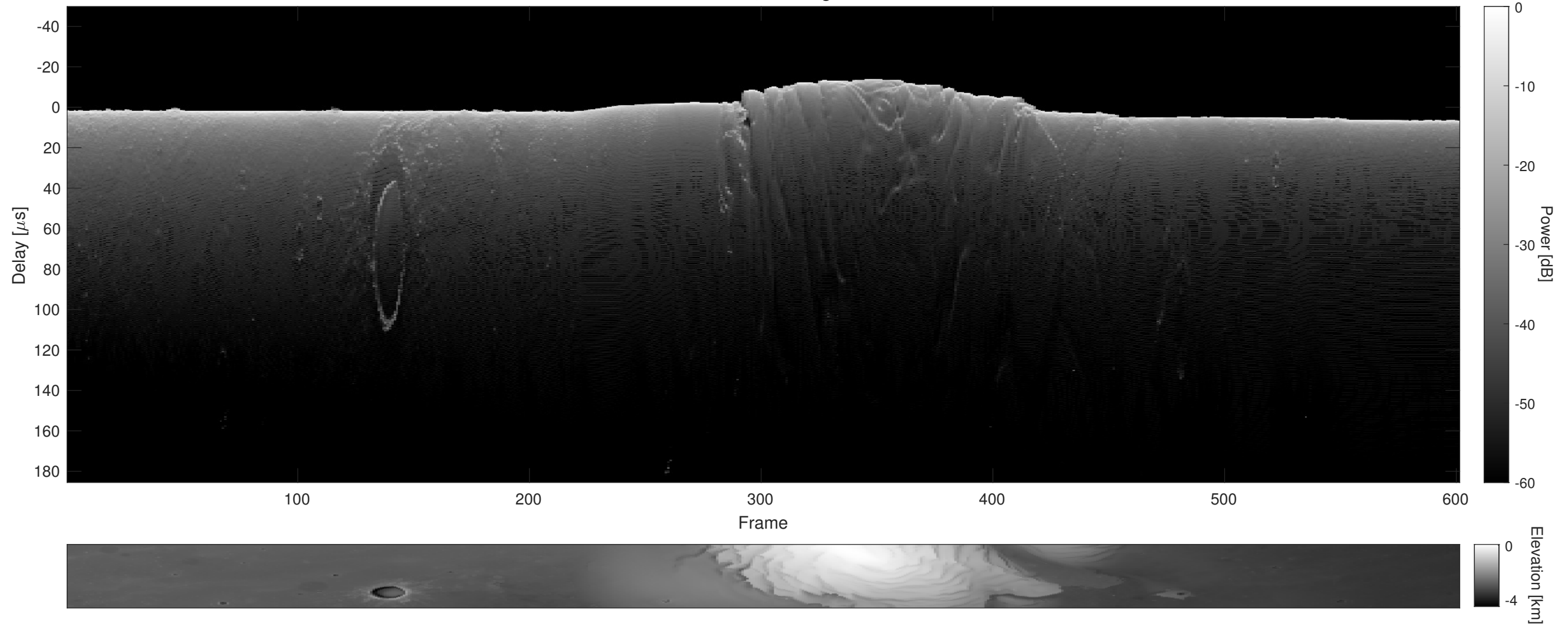
Orbit 18037, Cluttergram
