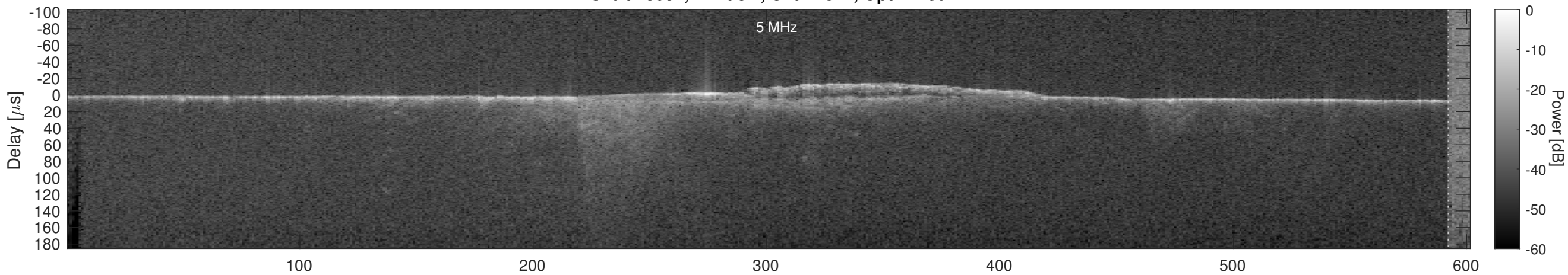
Orbit 18037, Cluttergram
