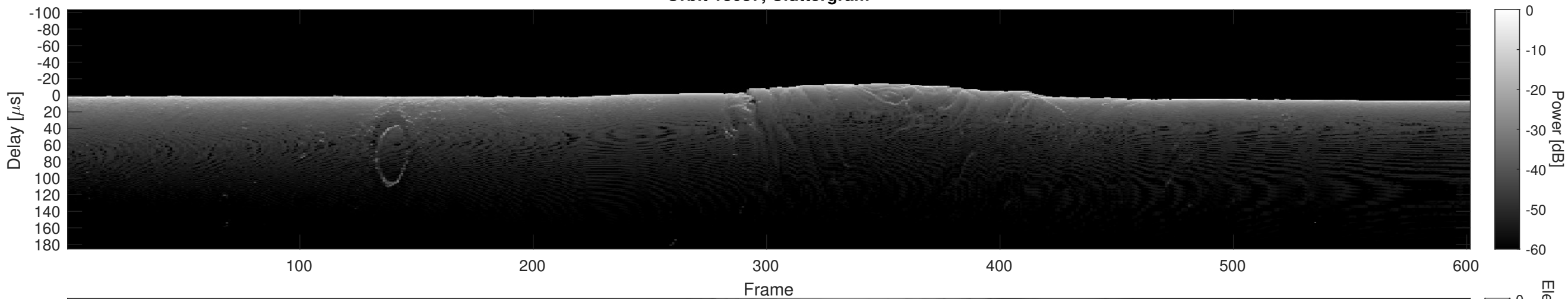
Orbit 18037, Cluttergram
