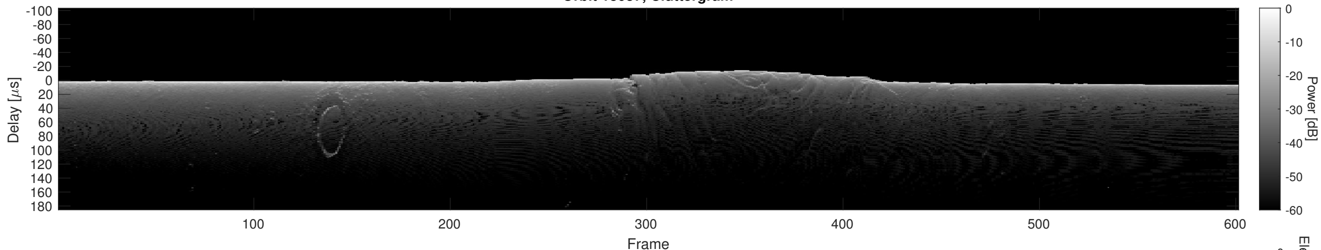
Orbit 18037, Cluttergram
