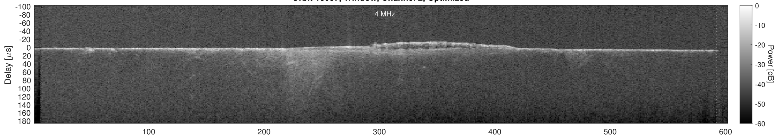
Orbit 18037, Cluttergram
