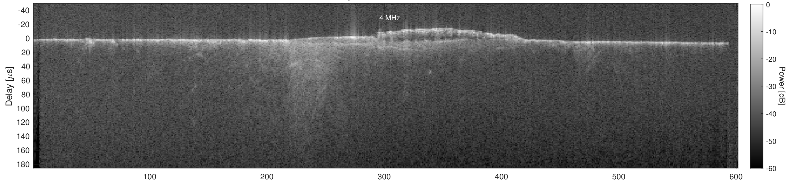
Orbit 18037, Cluttergram
