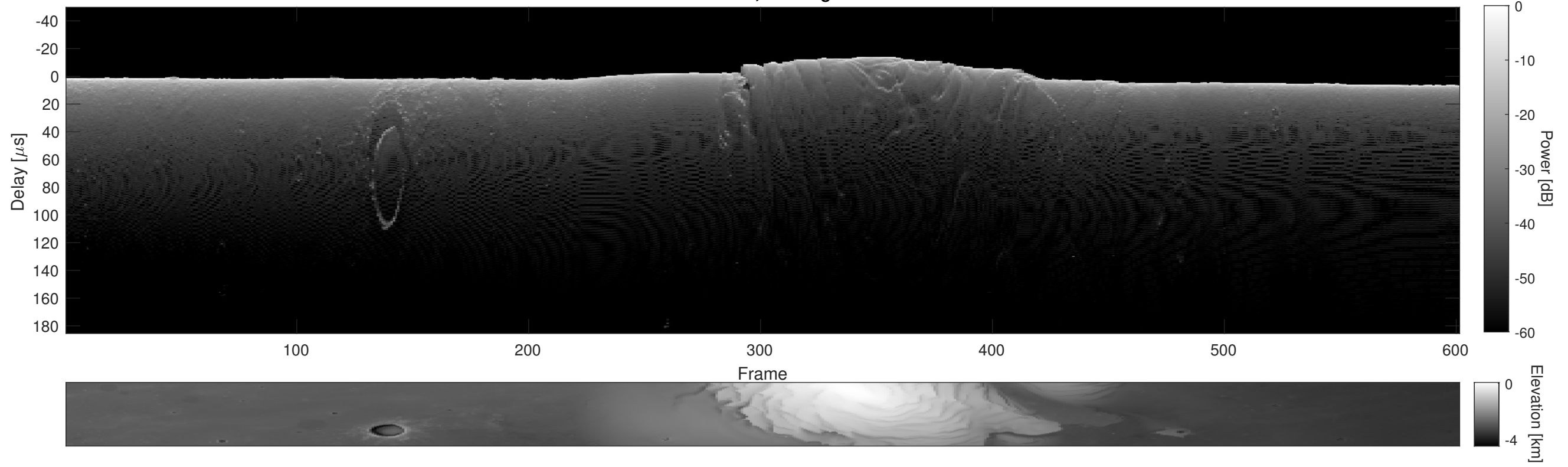
Orbit 18037, Cluttergram
